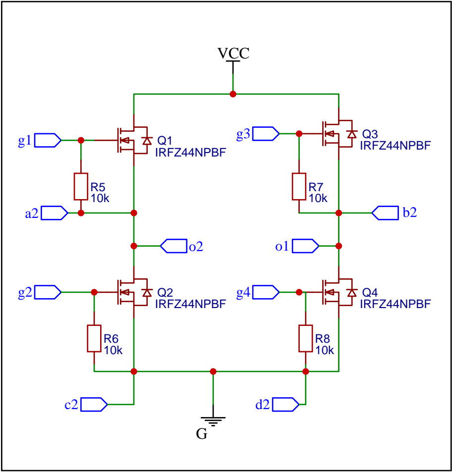
Switching Circuit
