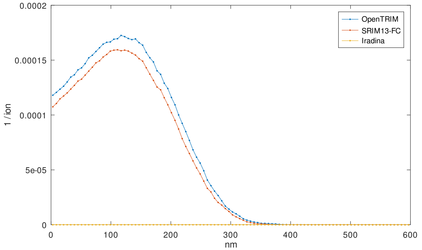
Phonon energy fraction \Delta E_{Ph}/E_0 by Fe ion
