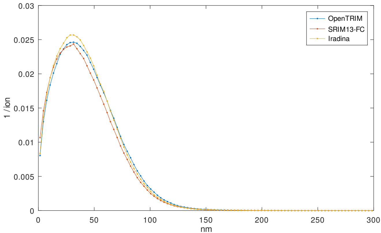
Total Phonon energy fraction \Delta E_{Ph}/E_0
