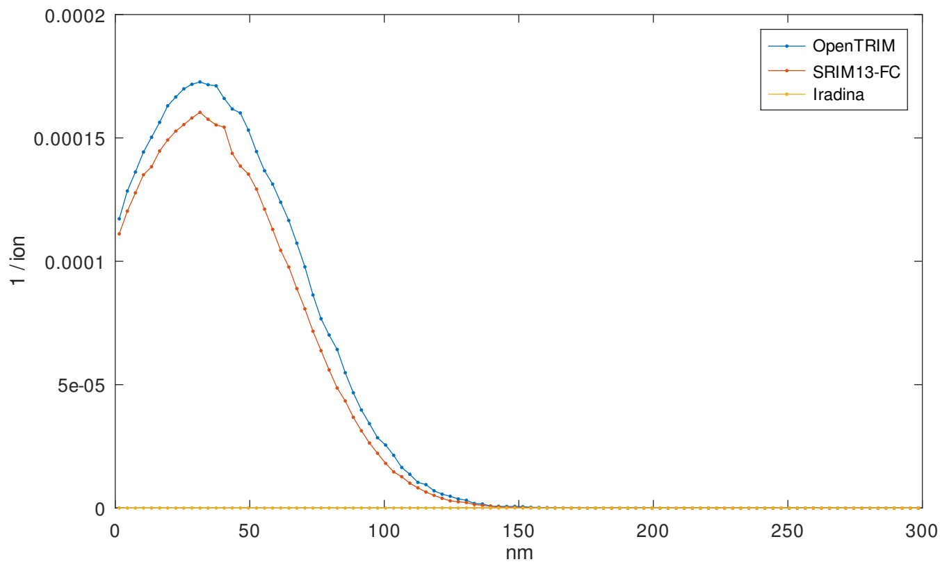
Phonon energy fraction \Delta E_{Ph}/E_0 by Xe ion
