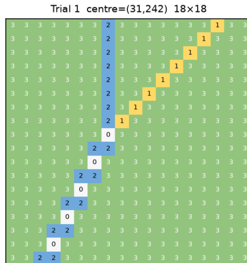
Figure 3.3: Intersection of (1, 1) and (0, 1) , yielding (1, 2) .
