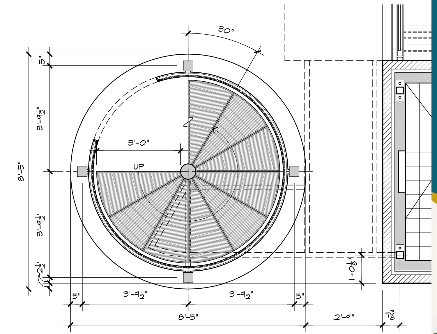
12 FIRST FLOOR PLAN SCALE: 1/2" = 1'-0"
