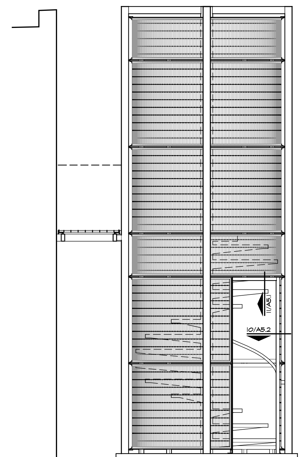
2 ELEVATION/SECTION SCALE: 3/8" = 1'-0"
