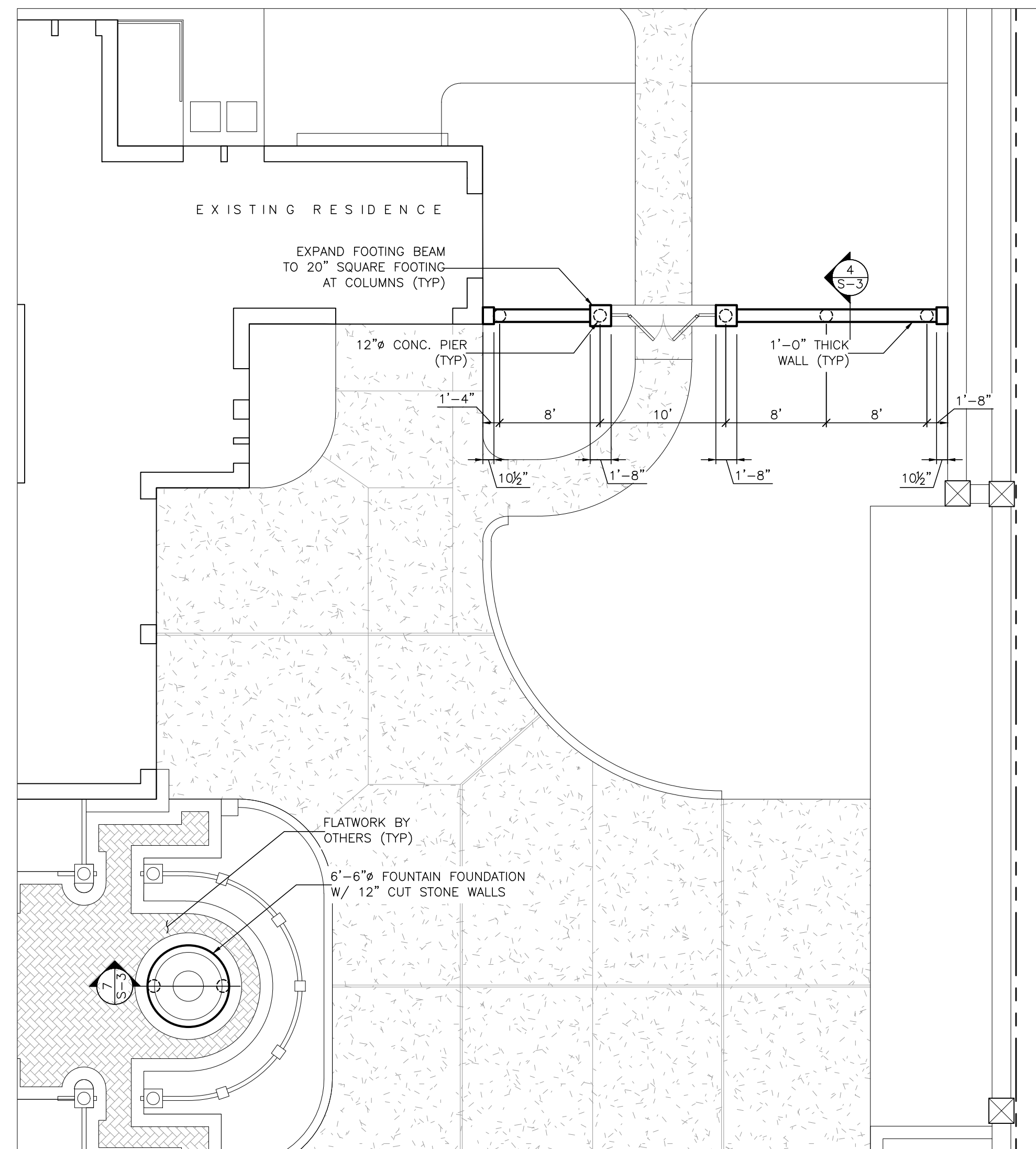
ENTRY ARBOR PLAN – SOUTH SCALE: 1/8" = 1'-0"
