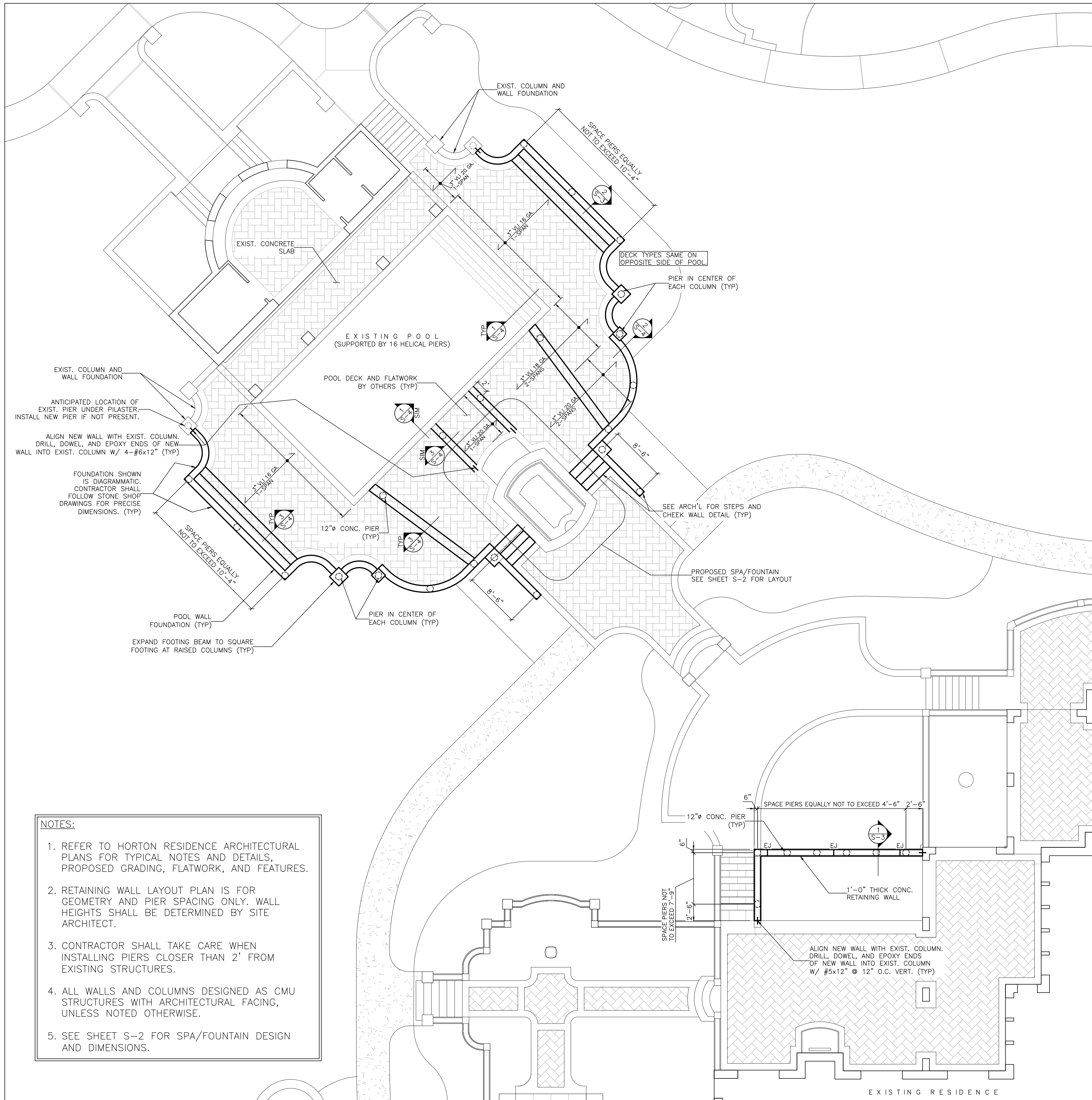
SITE RETAINING WALL AND POOL DECK LAYOUT PLAN – NORTH SCALE: 1/8" = 1'-0"
