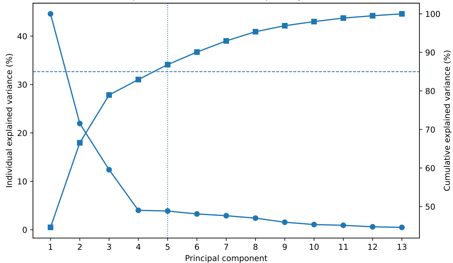
PCA explained variance — FRICTA primary indicators
