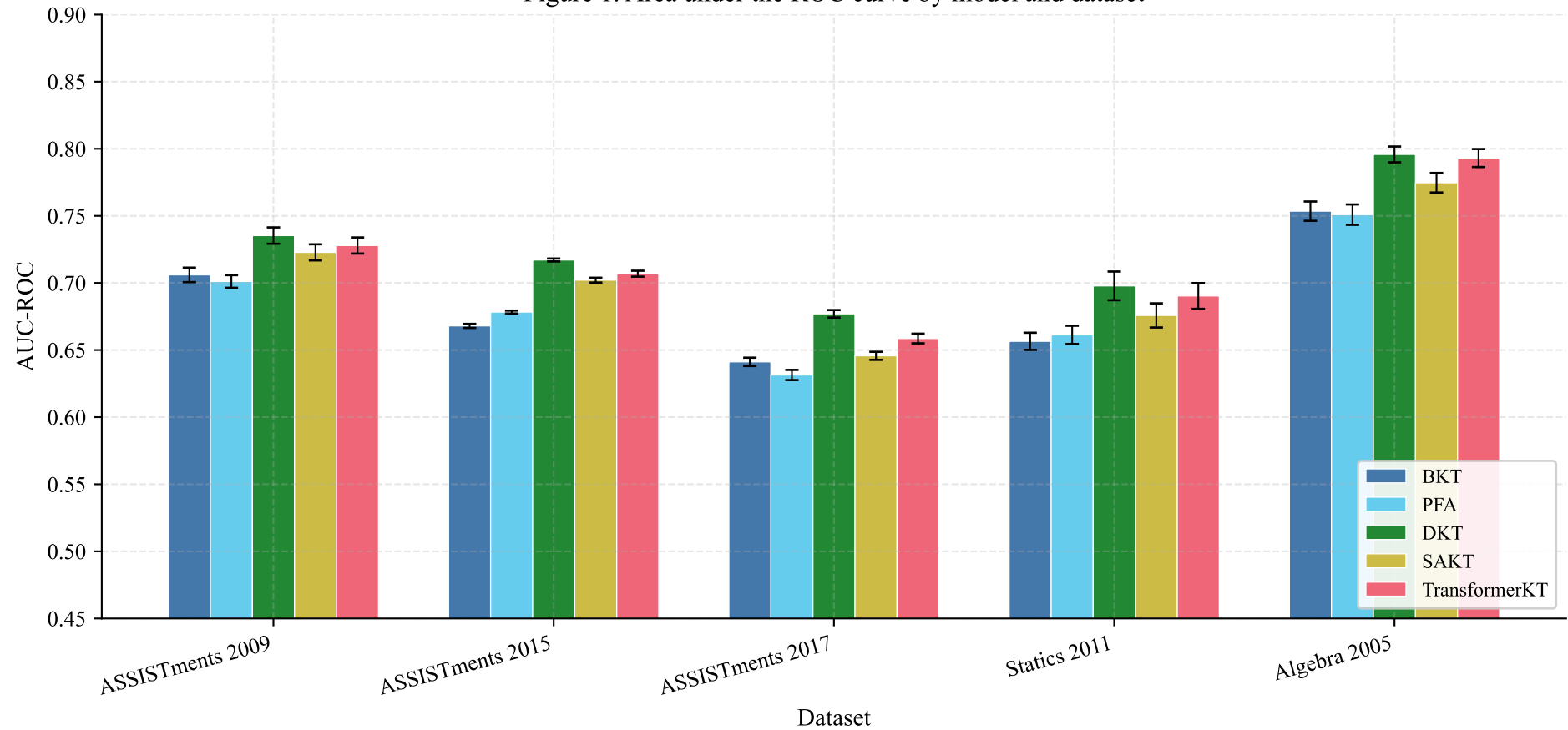
Figure 1. Area under the ROC curve by model and dataset
