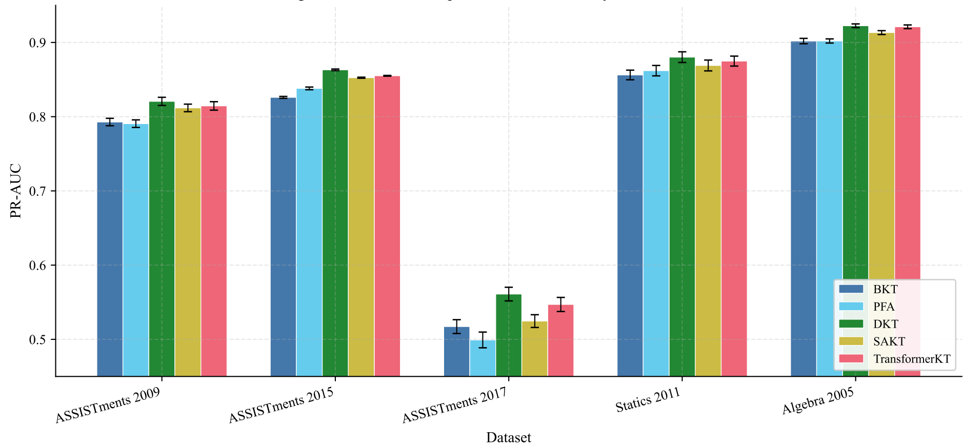
Figure 2. Area under the precision-recall curve by model and dataset
