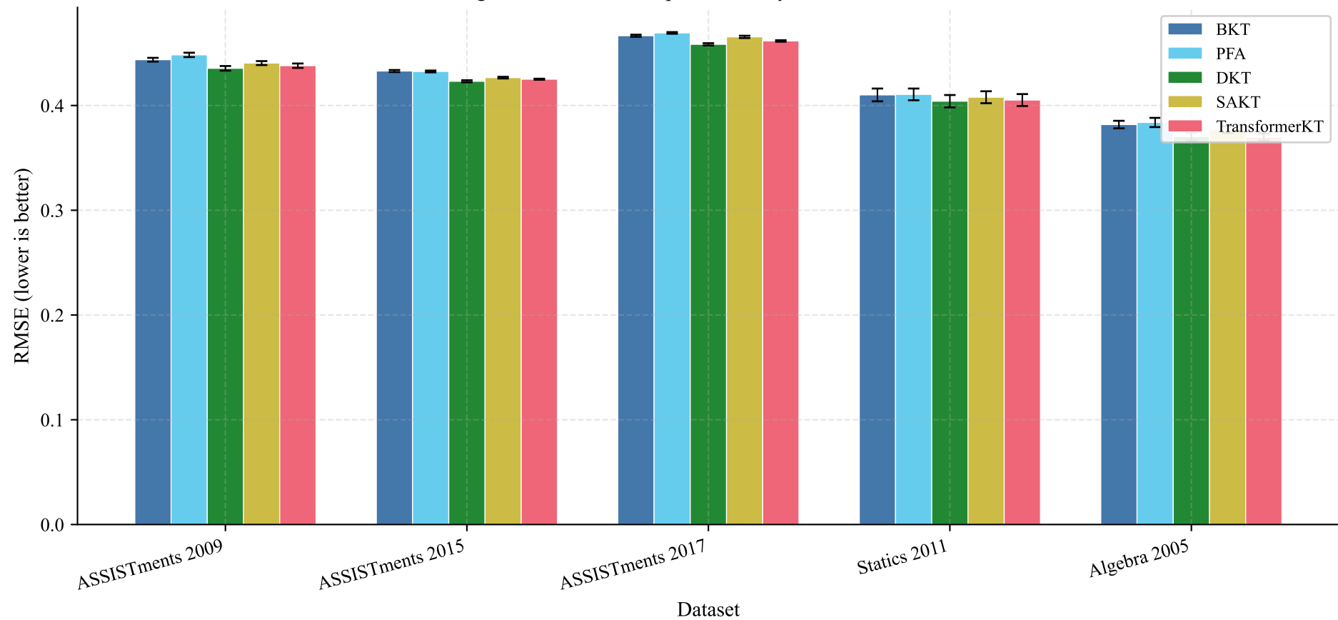
Figure 3. Root mean square error by model and dataset
