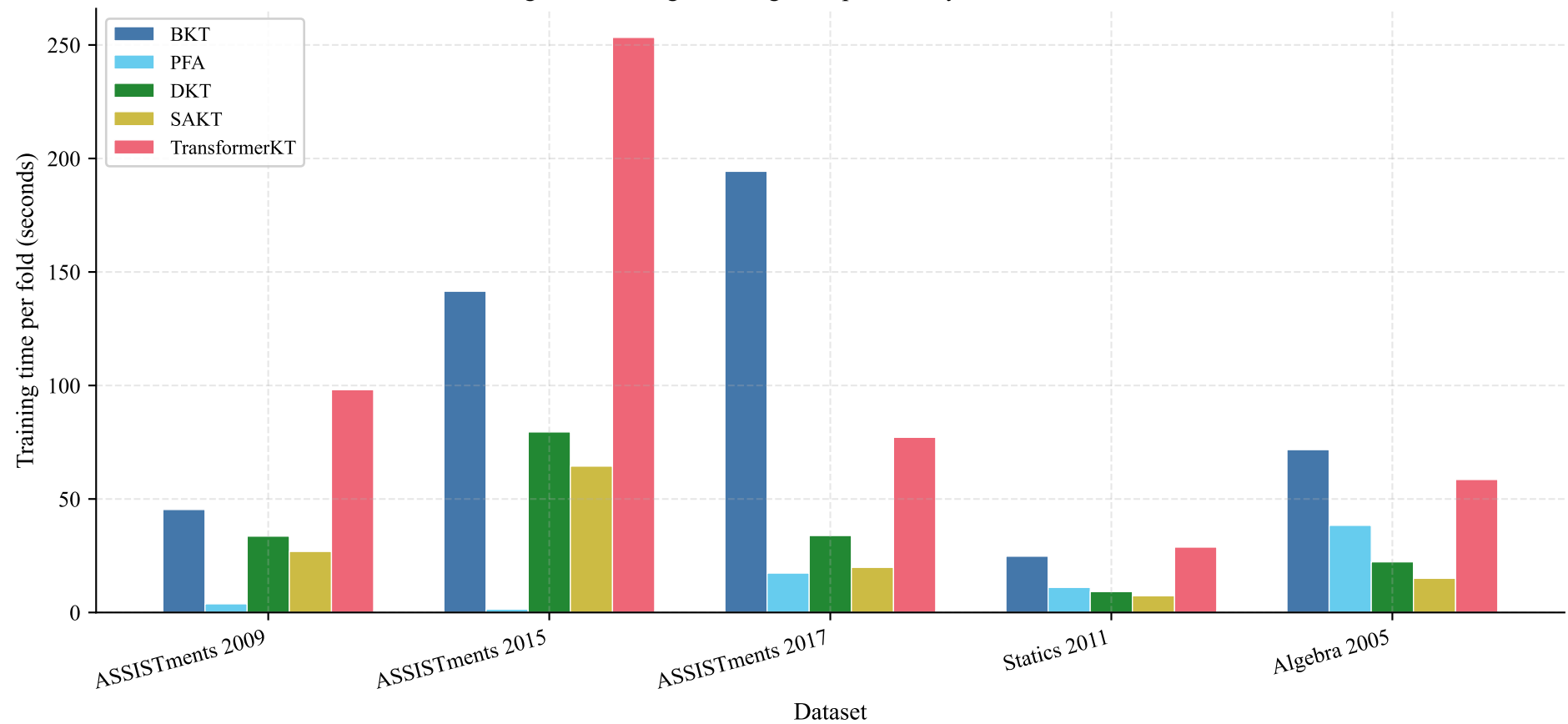
Figure 4. Average training time per fold by model and dataset
