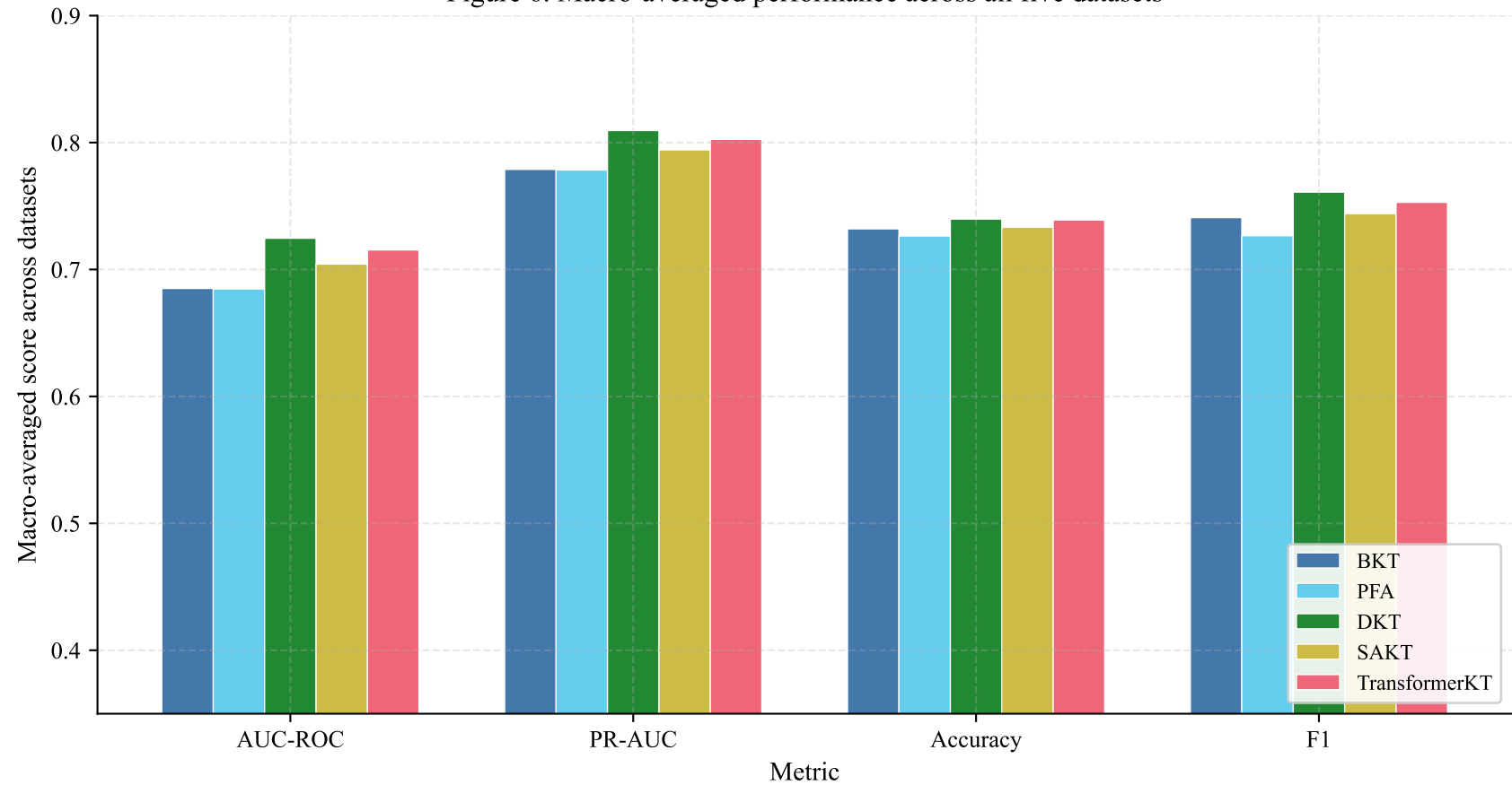
Figure 6. Macro-averaged performance across all five datasets
