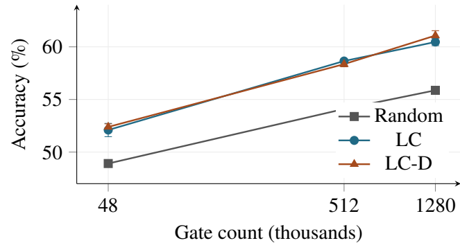
(a) Dense CIFAR-10 (T)
