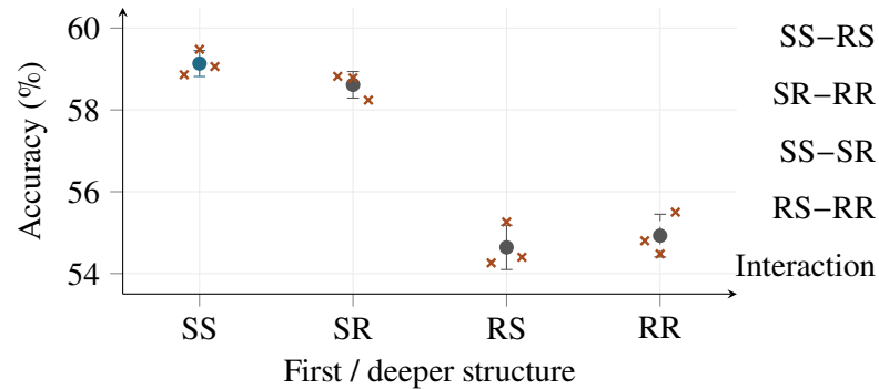
(a) Dense M factorial (V)
