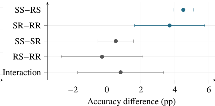
(b) Paired effects (V)
