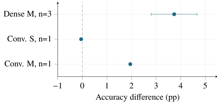
(a) Frozen CIFAR-10.1 tests
