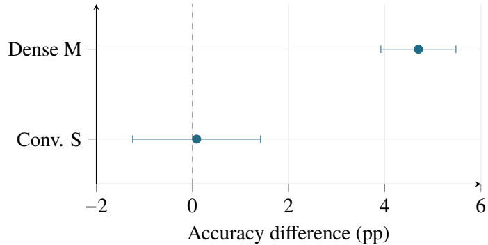
(a) Adapted WARP: LC minus random
