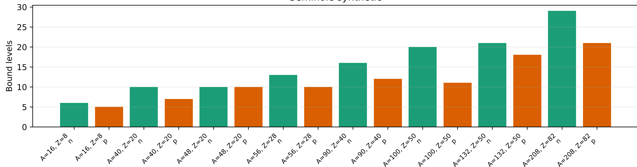
Wahlborn synthetic
