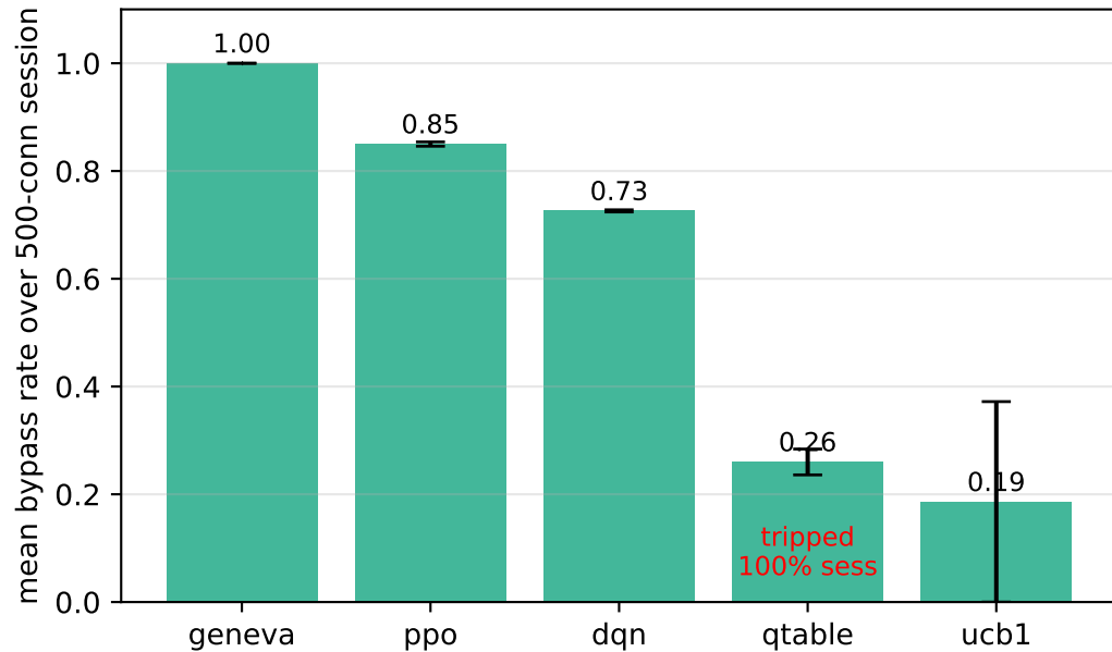
E6 — strict-graylist (5MB/60s) campaign (Iran-documented threshold)
