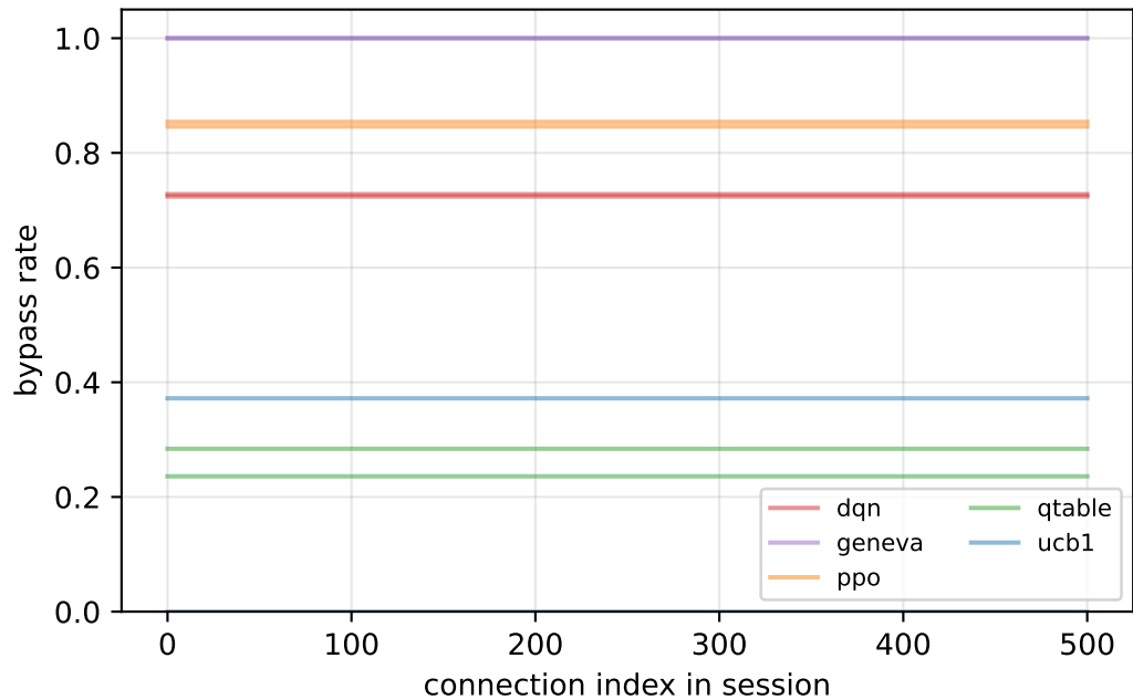
E6 — per-session bypass rate (lines per session)
