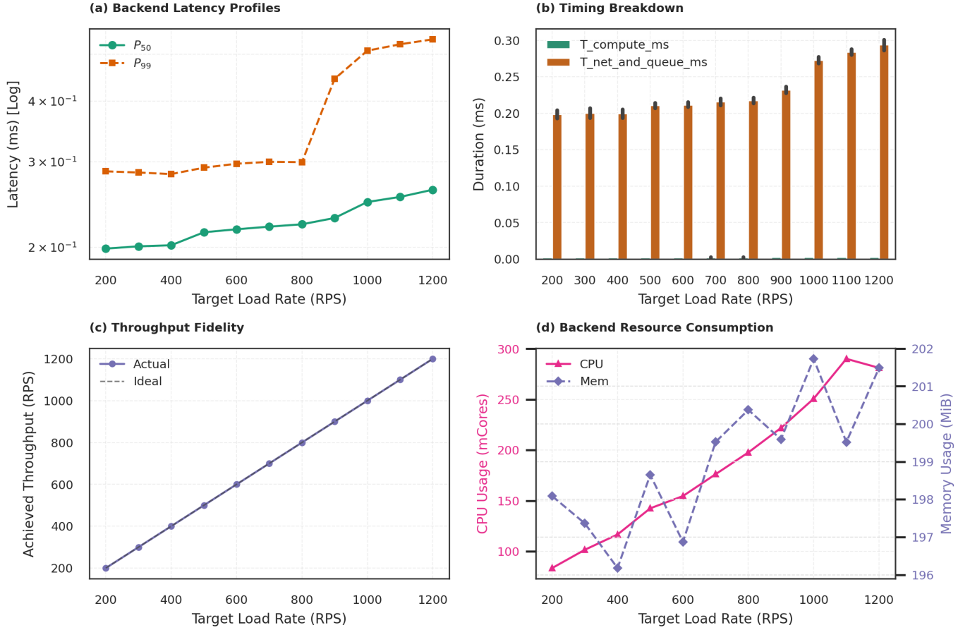
FIGURE 6. Baseline performance evaluation of backend service that evaluate directly to the backend server using ghz tool with gRPC load request: (a) median and tail latency ( p_{50}, p_{99} ); (b) compute vs net and queue time latency ( t_{comp}, t_{net\_queue} ); (c) systems throughput; (d) resource utilization (CPU and Memory). These graphs are represent the result correspond to the evaluation scenario B on Fig. ??.
