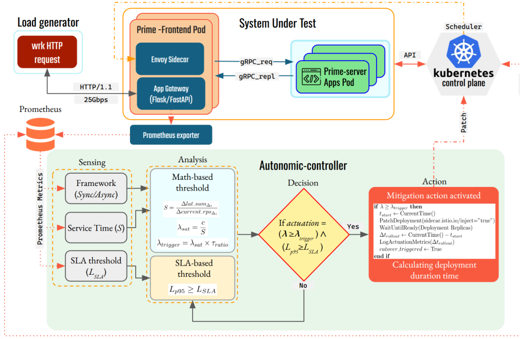
FIGURE 3: The proactive autonomic controller architectures.
