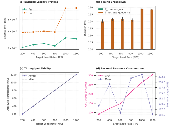
FIGURE 6. Baseline performance evaluation of backend service that evaluate directly to the backend server using ghz tool with gRPC load request: (a) median and tail latency ( p_{50} , p_{99} ); (b) compute vs net and queue time latency ( t_{comp} , t_{net\_queue} ); (c) systems throughput; (d) resource utilization (CPU and Memory).
