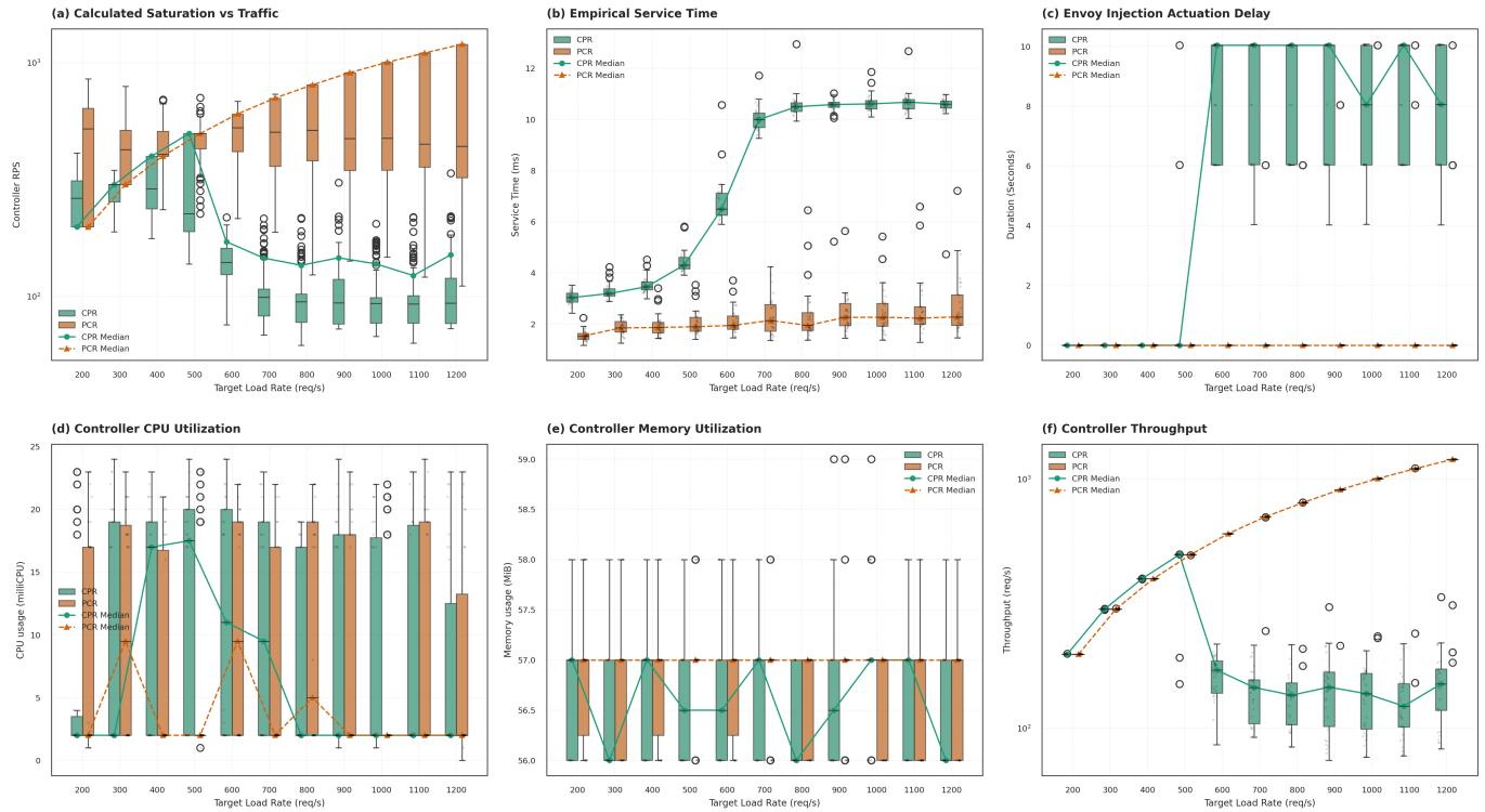
FIGURE 8. Autonomic controller performance evaluation in synchronous mode (Flask/Gunicorn): (a) Calculated saturation point ( \lambda_{sat} ); (b) service time ( S ); (c) Actuation time when envoy deployed to frontend pods; (d) controller cpu utilization; (e) controller memory utilization; (f) controllers throughput.
