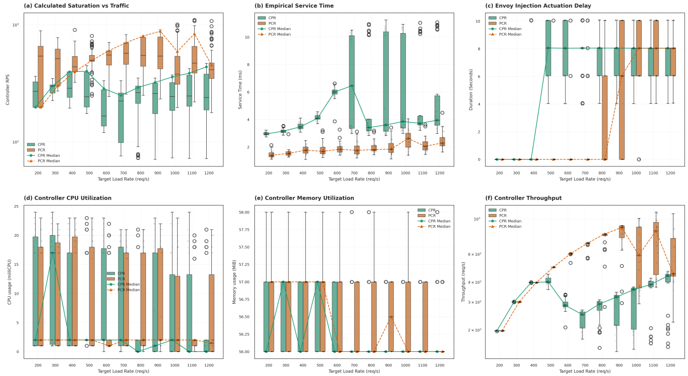
FIGURE 7. Autonomic controller performance evaluation in asynchronous mode (FastAPI/Uvicorn): (a) Calculated saturation point ( \lambda_{sat} ); (b) service time ( S ); (c) Actuation time when envoy deployed to frontend pods; (d) controller cpu utilization; (e) controller memory utilization; (f) controllers throughput.
