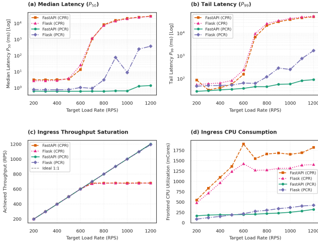
FIGURE 5. Baseline performance evaluation of frontend communication gateway (Synchronous and Asynchronous method) within Connection Per Request (CPR) and Persistent Connections Reuse (PCR) model: (a) median latency ( p_{50} ); (b) end-to-end latency ( p_{99} ); (c) systems throughput; (d) resource utilization (CPU).
