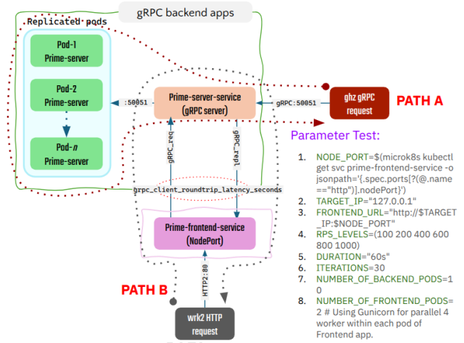
Figure 2: Evaluation mechanism to accurately examine the frontend (HTTP) and backend (gRPC) latency utilizing different benchmark tools.
