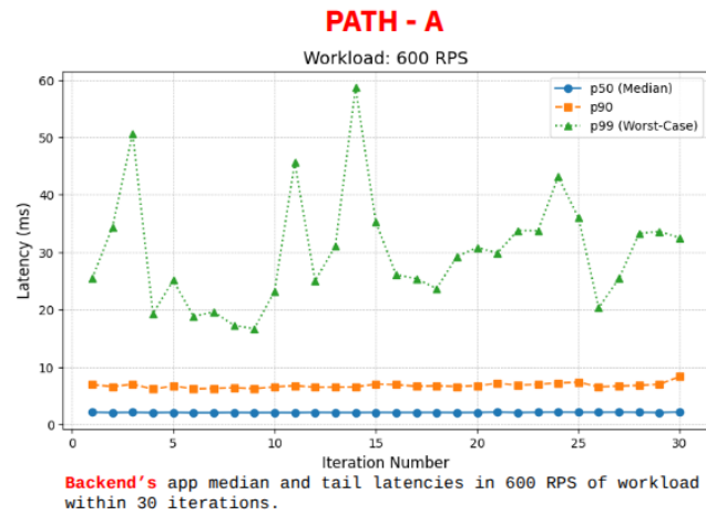
Figure 3: gRPC backend latency evaluation using ghz benchmark tool.
