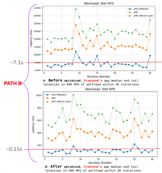
Figure 4: End-to-end frontend latency evaluation using wrk2 as workload generator. (A) Connection-Per-Request paradigm - Before optimized, (B) Persistent Channel Reuse paradigm - After optimized
