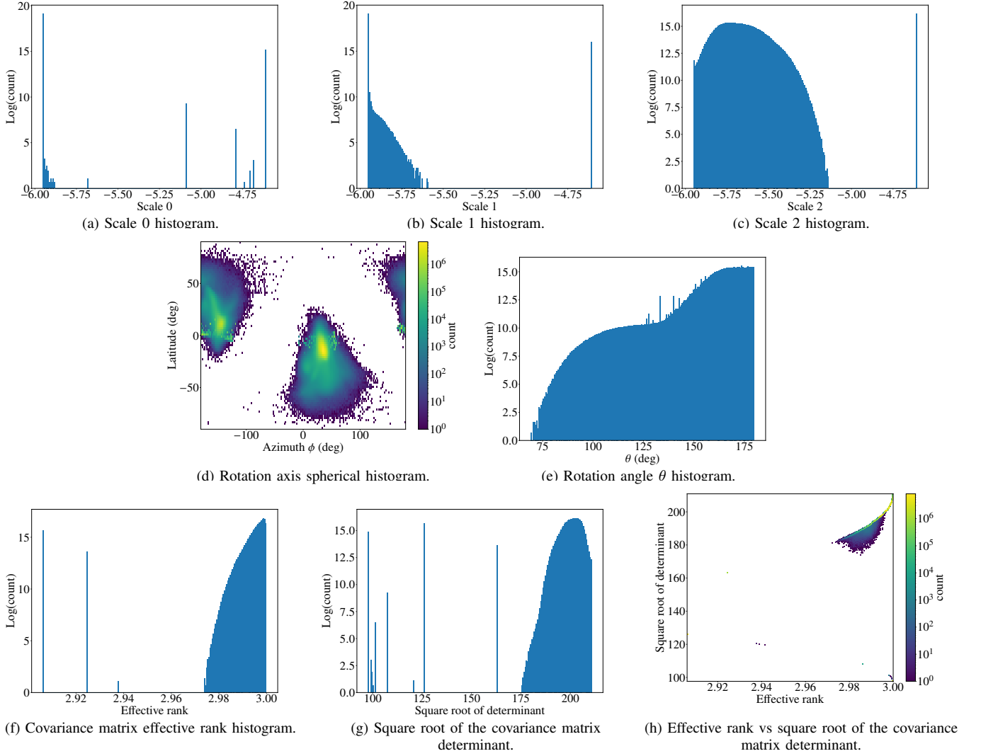
Fig. 5: Analysis of the Gaussian splats from Philipp's first dynamic reconstruction.
