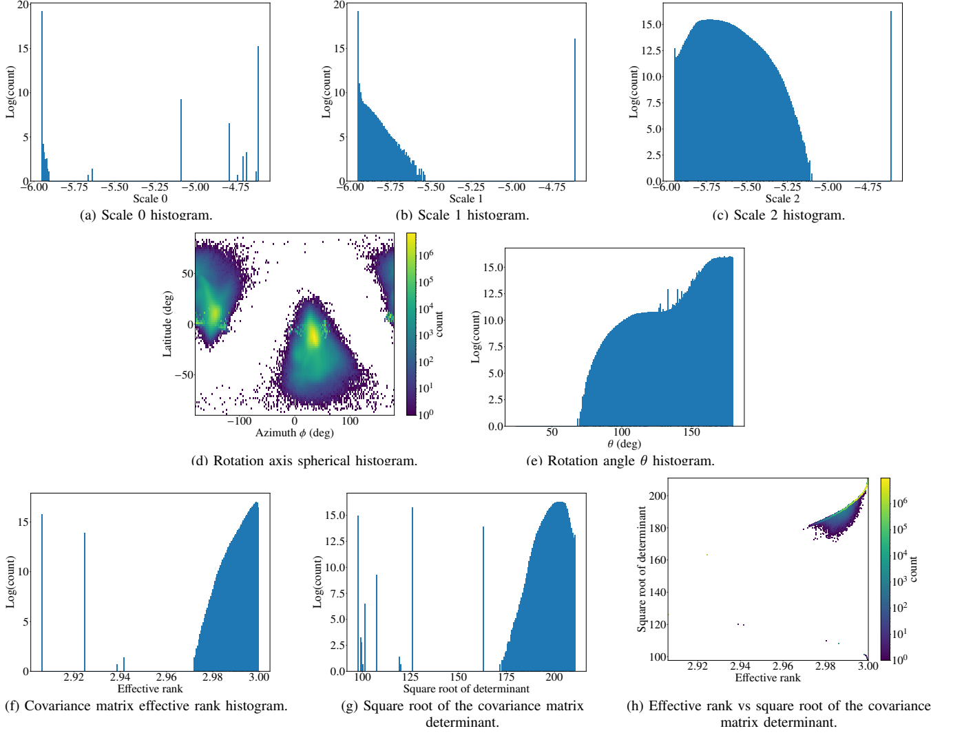
Fig. 6: Analysis of the Gaussian splats from Philipp's second dynamic reconstruction.
