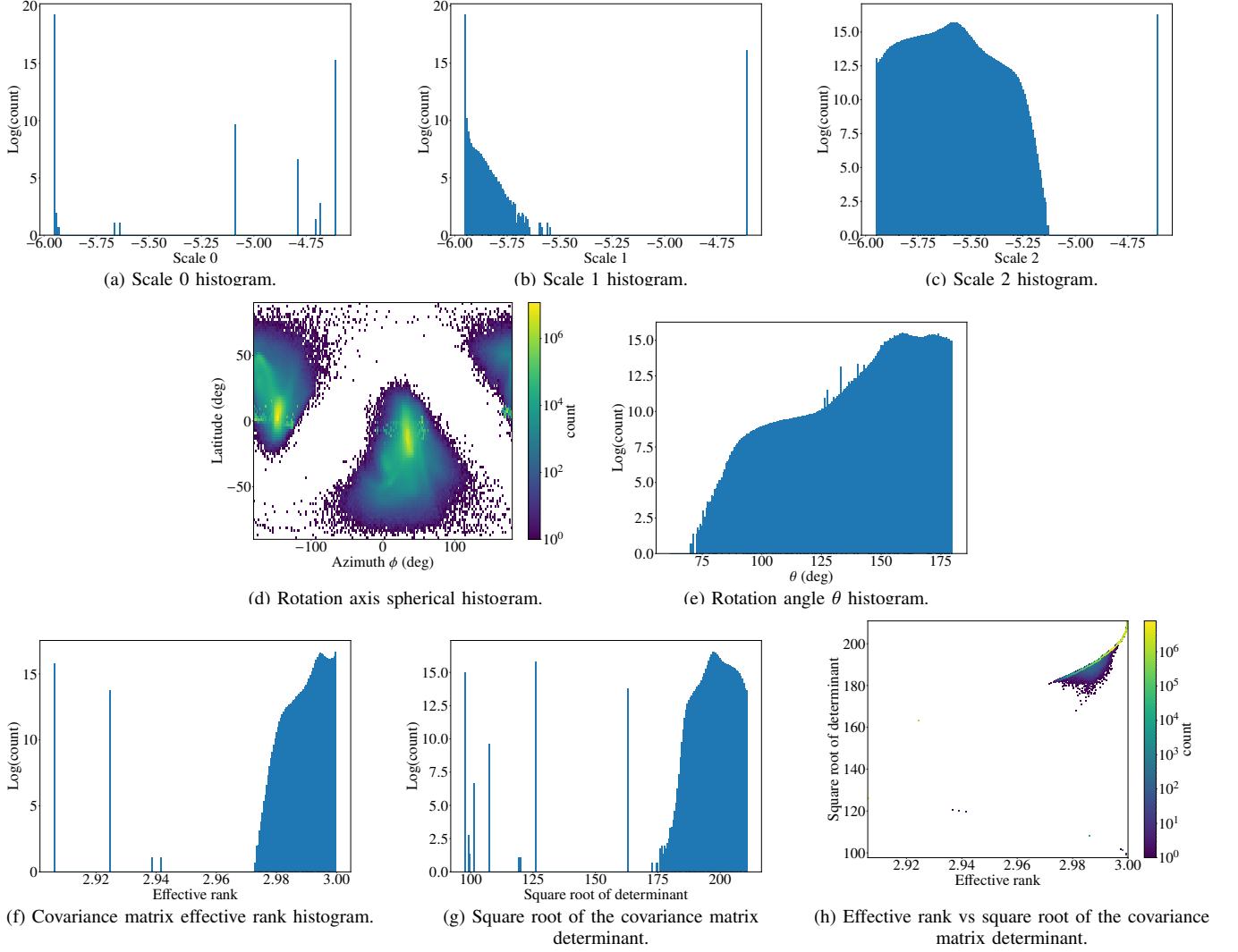
Fig. 8: Analysis of the Gaussian splats from Thanos's dynamic reconstruction.
