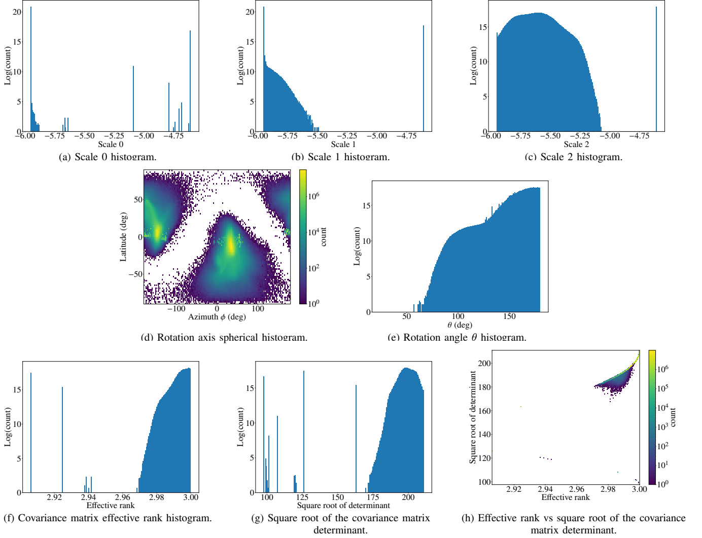
Fig. 2: Analysis of the Gaussian splats from all dynamic reconstructions.
