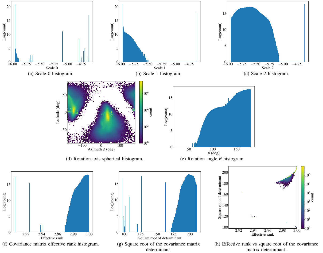
Fig. 2: Gaussian splat analysis of all dynamic reconstructions.
