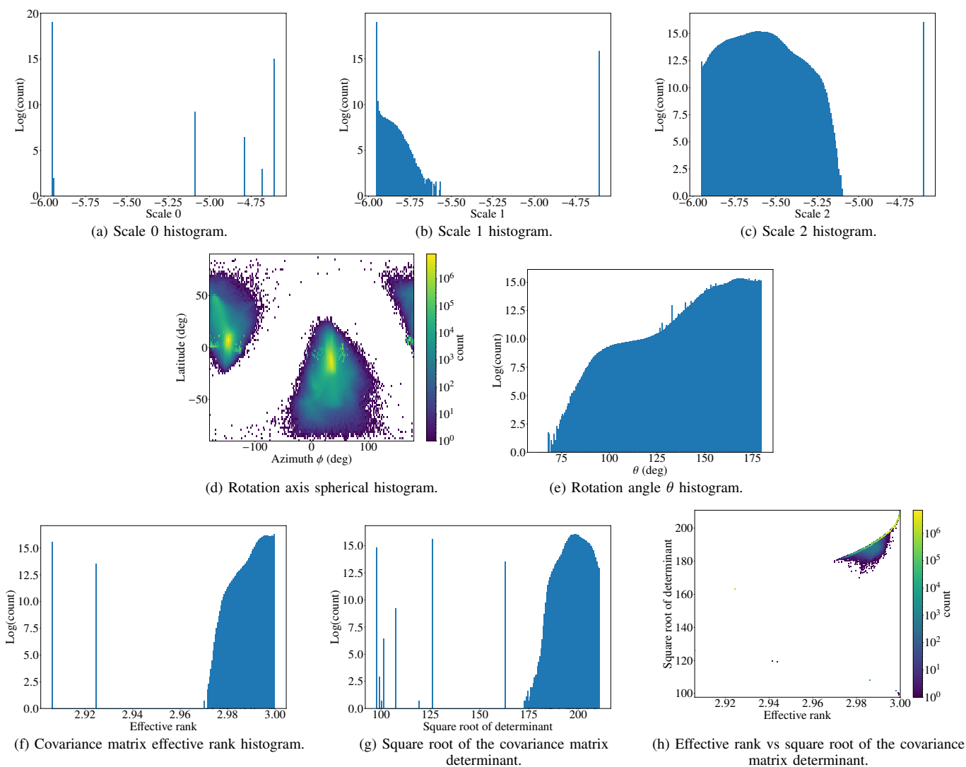
Fig. 7: Gaussian splat analysis of Simone's dynamic reconstruction.
