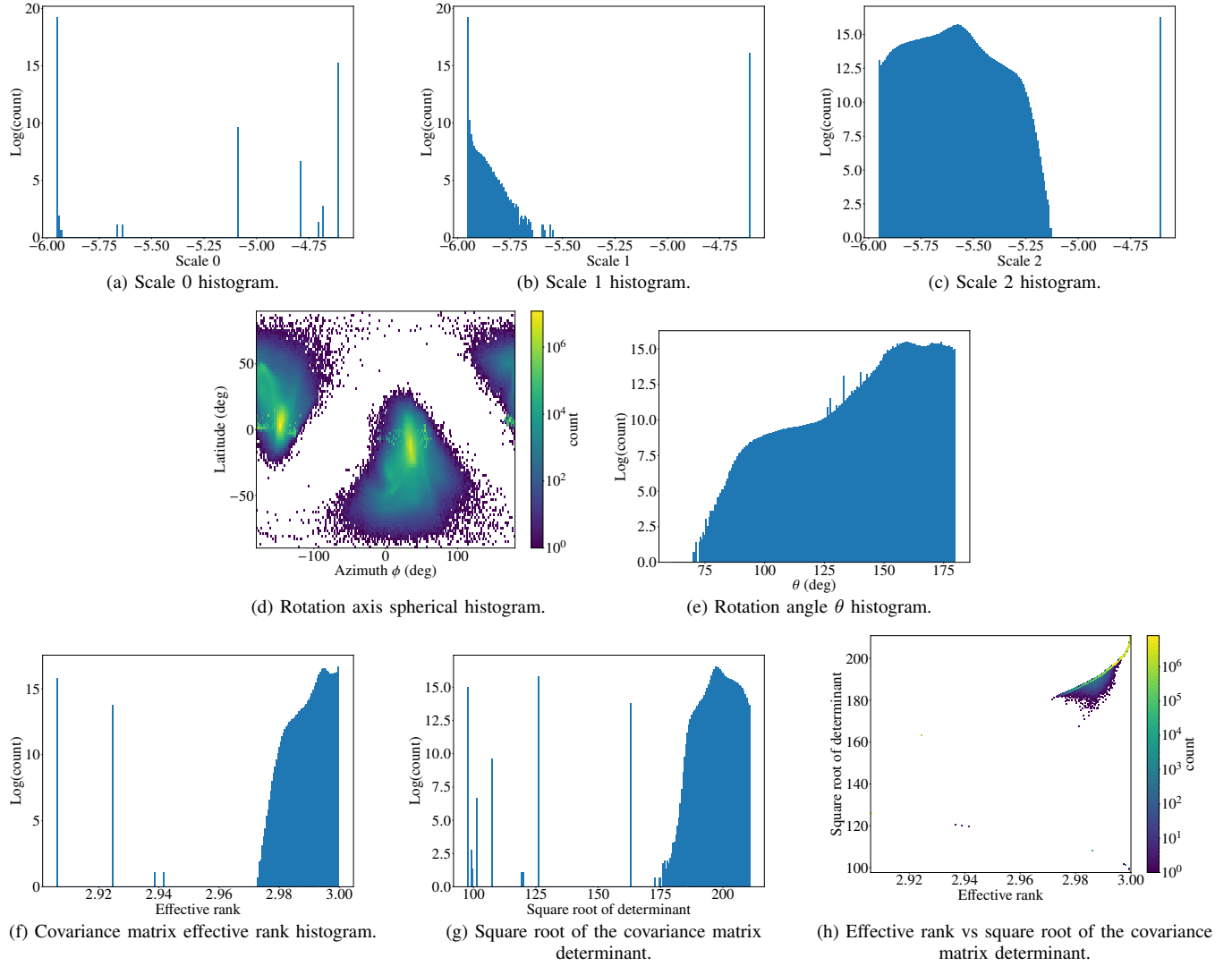
Fig. 8: Gaussian splat analysis of Thanos's dynamic reconstruction.
