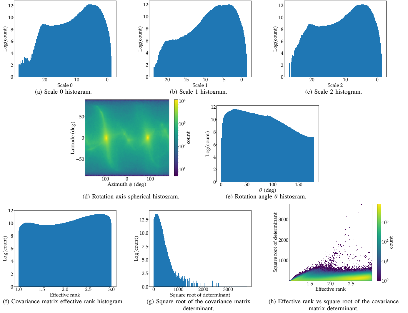
Fig. 11: Gaussian splats analysis from all static reconstructions.
