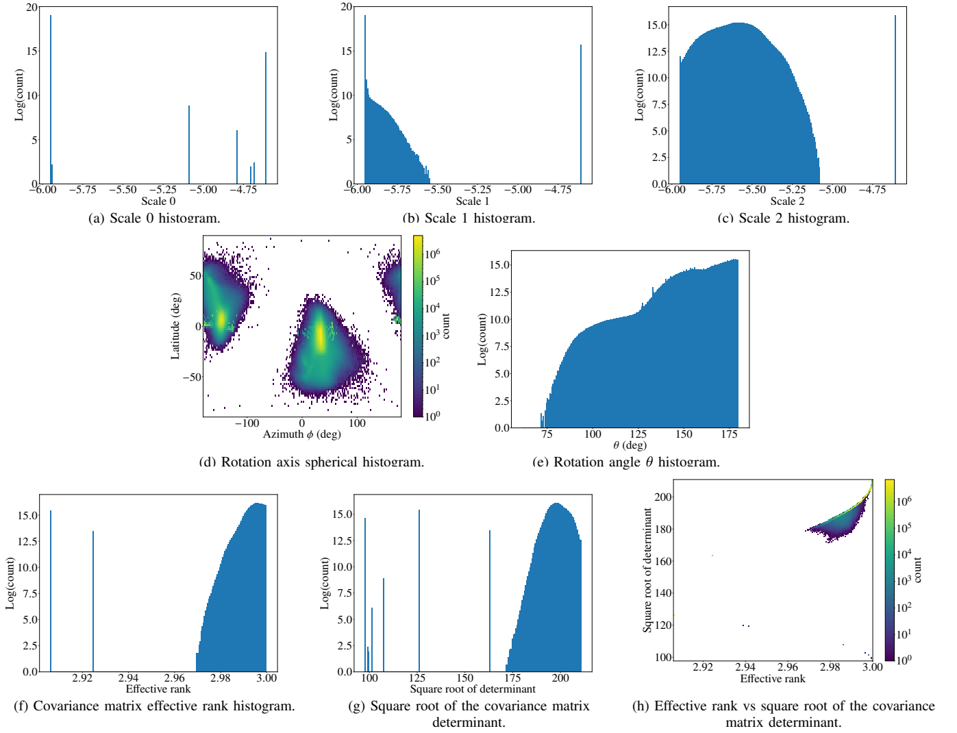
Fig. 4: Gaussian splats analysis of Nathalie's dynamic reconstruction.
