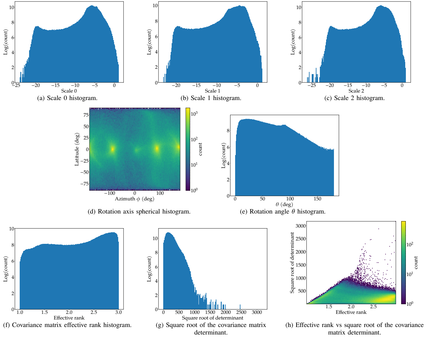
Fig. 13: Gaussian splat analysis of the Chapel static reconstruction.
