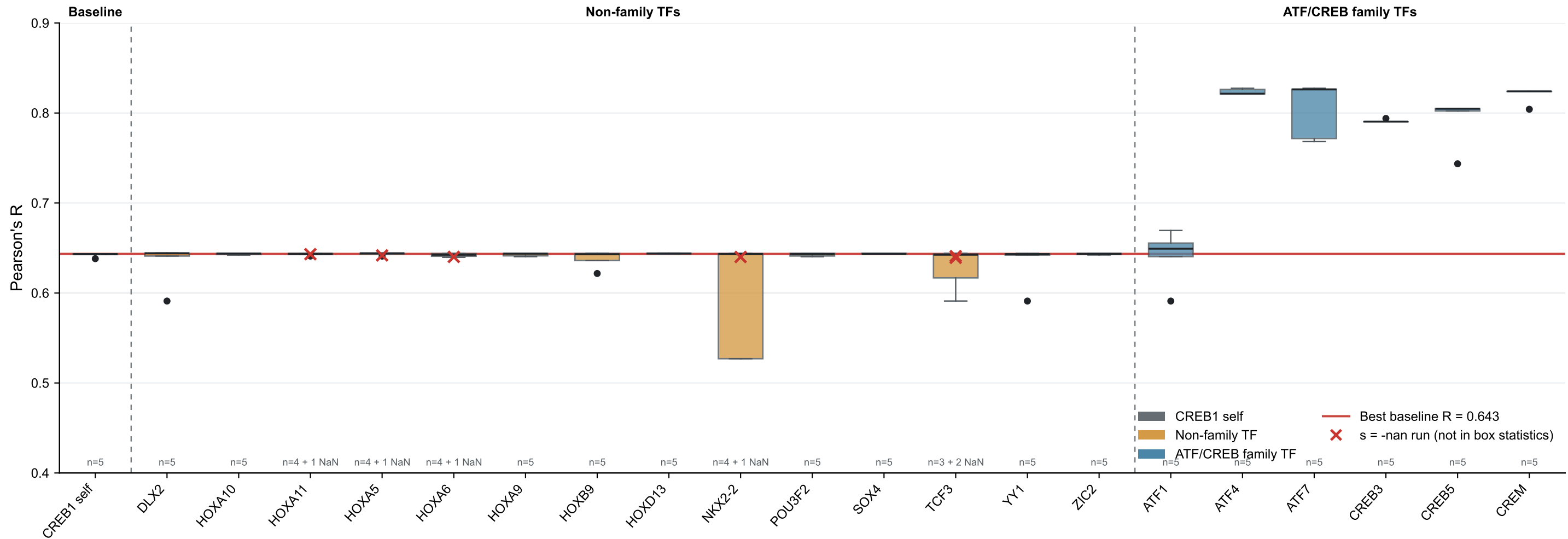
Figure 3A | Effect of adding family and non-family TFs
