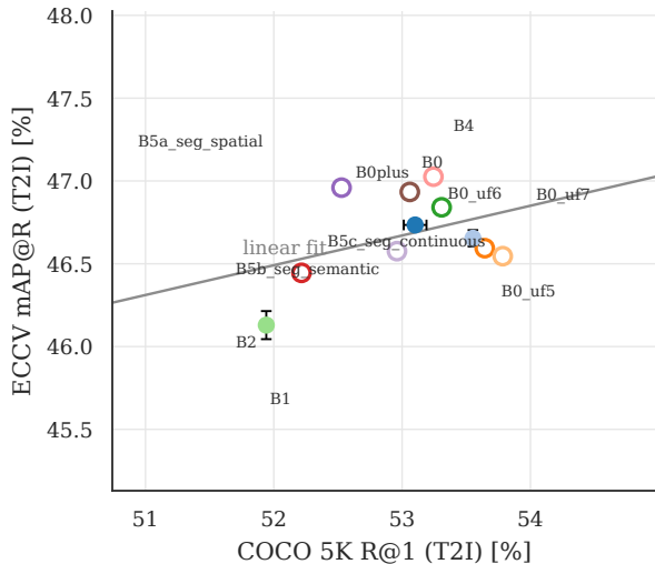
Text-to-Image
