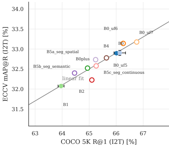
Image-to-Text
