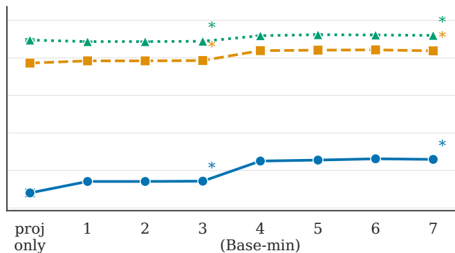
Text-to-image
