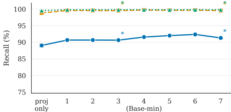
Image-to-text
