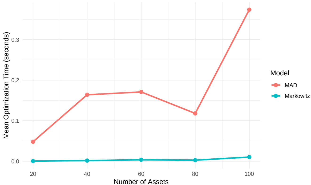
Computational Scaling with Asset–Universe Size
