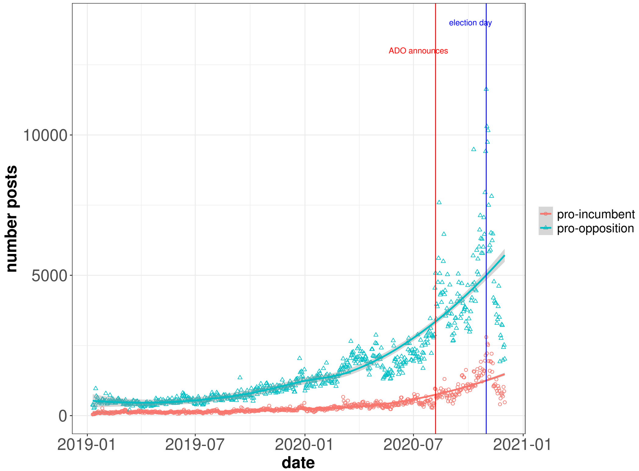
Distribution of Posts Over Time (Days)
