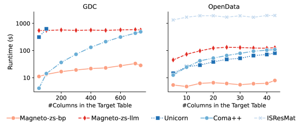
Figure 8: Runtime analysis (log-scale y-axis). Magneto scales well with large datasets: Magneto-zs-bp is often much faster than baselines, while Magneto-zs-llm maintains consistent runtimes, finishing large tasks within minutes. ISResMat and Unicorn fail to complete GDC after 100 columns.
