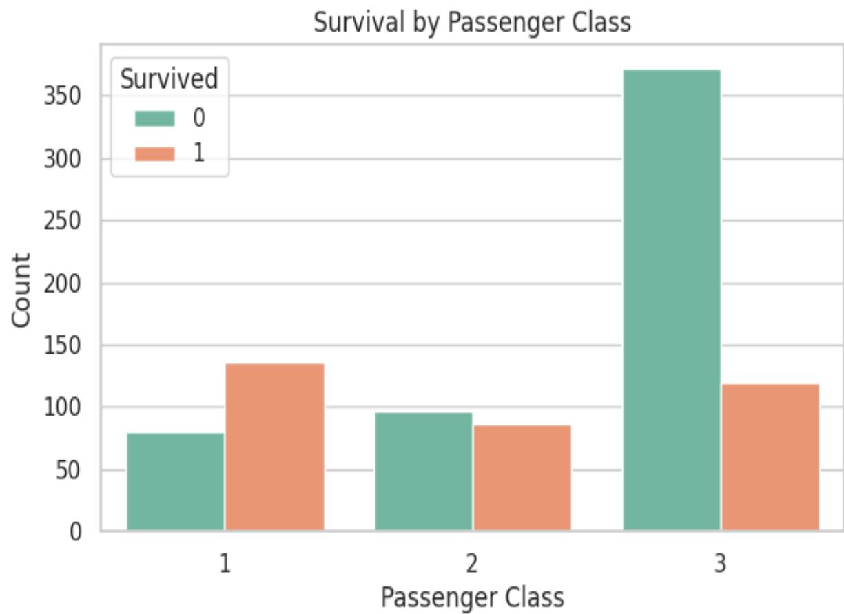
Countplot of Survived
