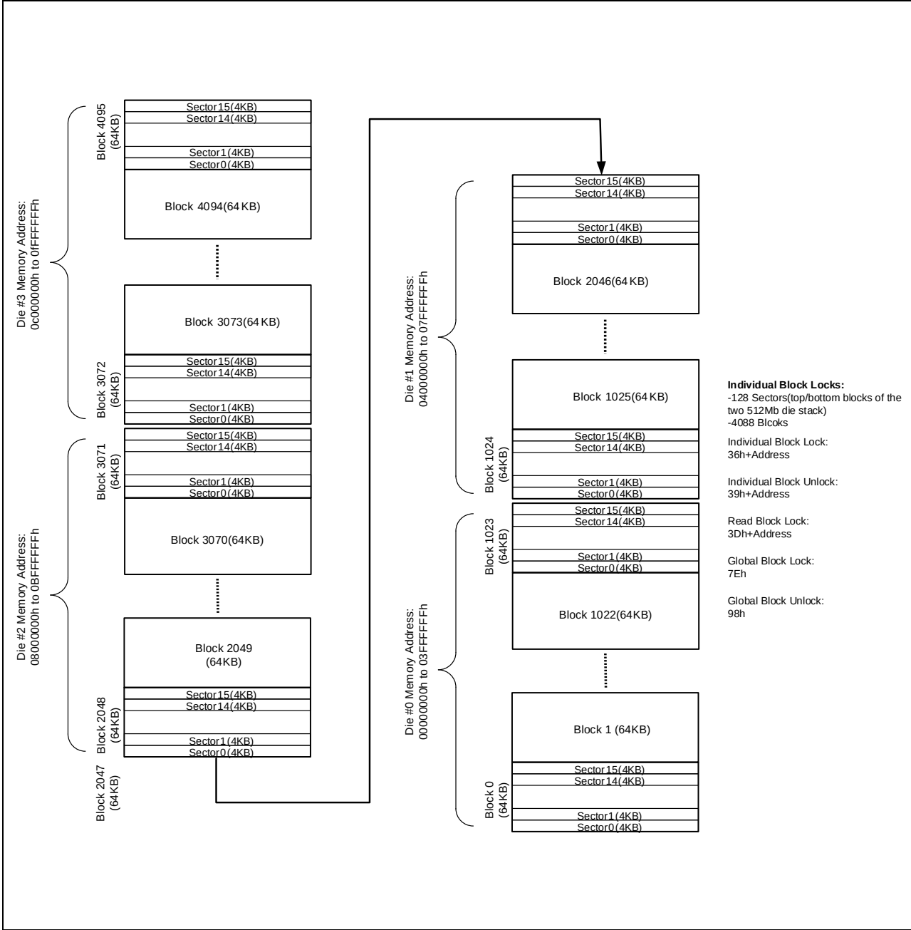
Figure 4d. Individual Block/Sector Locks
