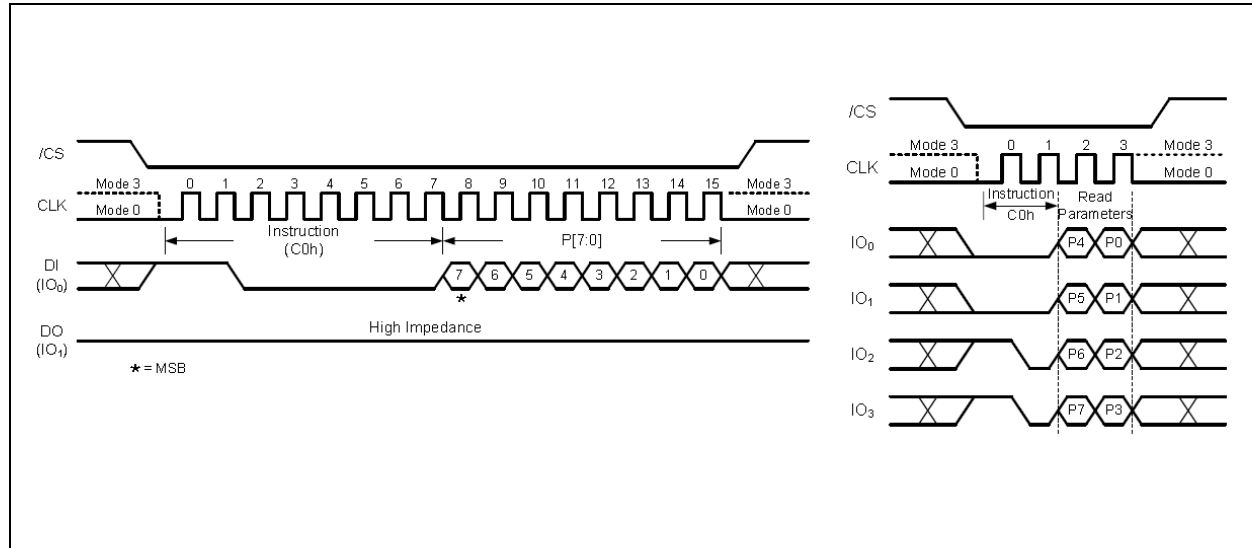
Figure 31. Set Read Parameters Instruction for SPI Mode (left) or QPI Mode (right)
