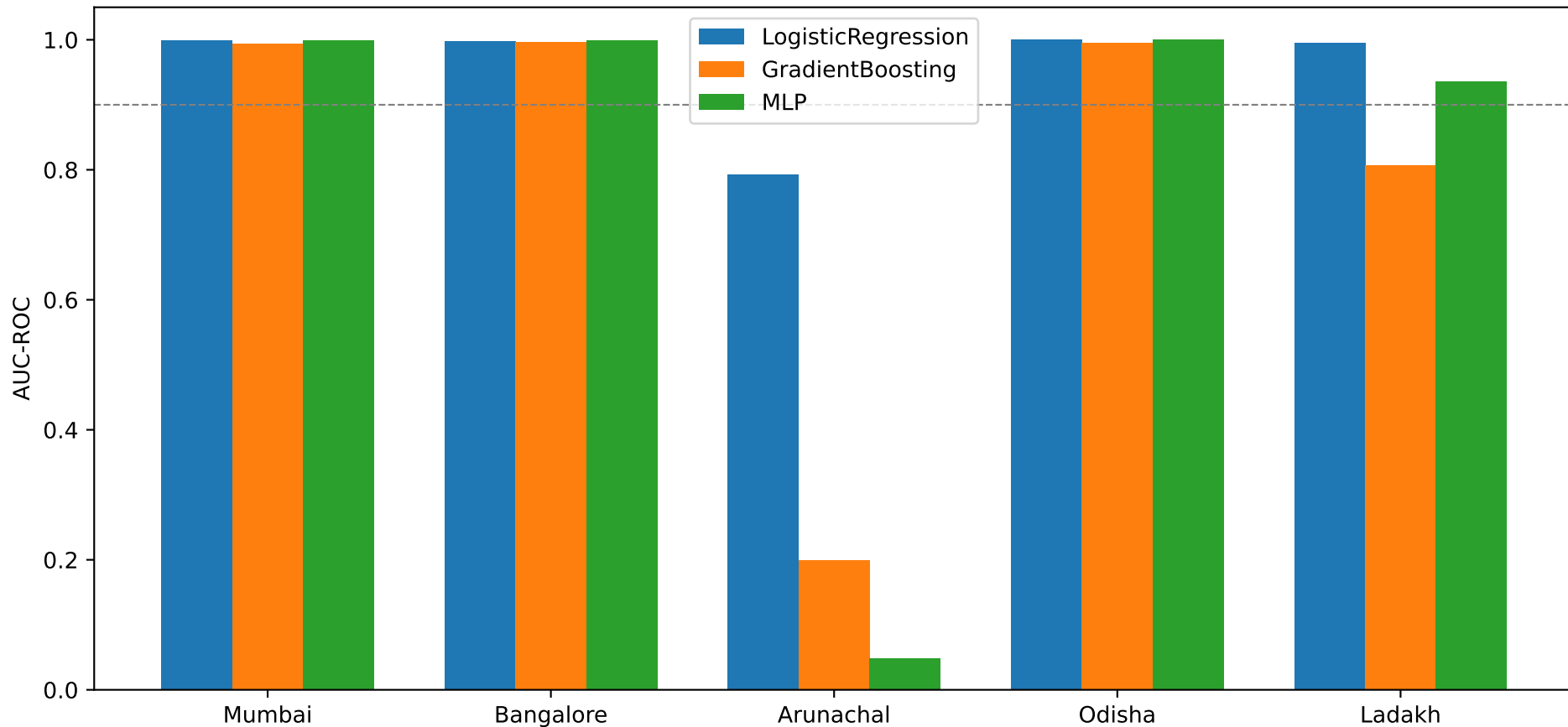
T1: Risk Classification AUC-ROC — Cross-Region Comparison
