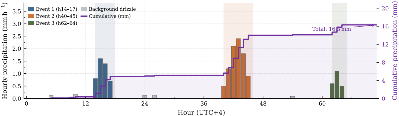
72-h hourly precipitation for Baku, Azerbaijan (Open-Meteo, March 2026). Three identified rain events are highlighted.
