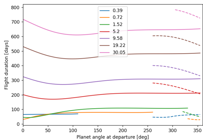
Fig. 2. Flight times in days versus initial polar angle at departure.
