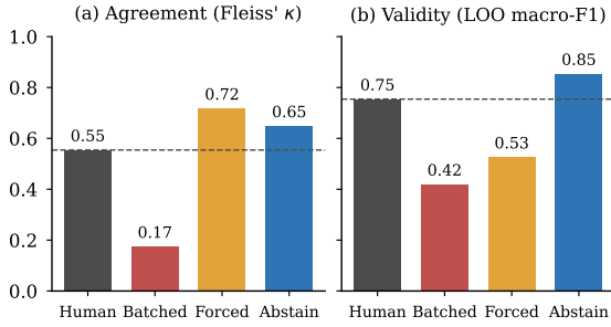
Figure 1: Agreement is not validity. (a) Mean Fleiss’ \kappa among three native speakers and among three LLMs under each protocol. (b) Mean macro-F1 against leave-one-annotator-out references for a held-out native speaker and the LLM majority vote. Dashed lines mark the human level.
