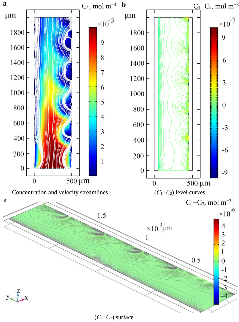
Fig. 9. The same as in Fig. 8; the results of simulation at |\Delta\phi| = 1.25 \text{ V} , t = 250 \text{ s} ; the beginning of section 4 in CVC (Fig. 7), formation of unstable vortices on the entire surface of the AEM.
