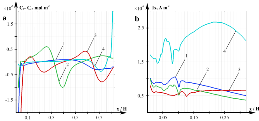
Fig. 12. Distributions of the space charge density (divided by F ), (C_1 - C_2) (a), and the normal component of the current density, I_x (b), in the cross-section of the channel at y=1450 \mu\text{m} . 1 – 594.0 s, 2 – 594.5 s, 3 – 595.0 s, 4 – 595.5 s.
