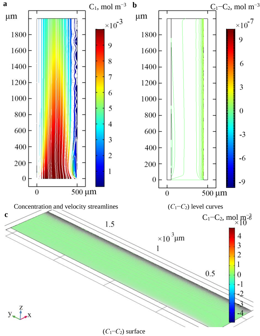
Fig. 8. Distribution of the cation concentration (shown with different color levels) and fluid velocity streamlines (white lines) (a) as well as the space charge density (divided by F ), C_1 - C_2 , presented with level curves (b) and surface of this function (c). Quasi-equilibrium regions at the membrane surface are not shown, since the concentration scale there is very different from the values outside these regions. The results of simulation at |\Delta\phi| = 0.625 V, t = 125 s; the beginning of section 3 in CVC (Fig. 7), formation of unstable vortices on the entire surface of the CEM.
