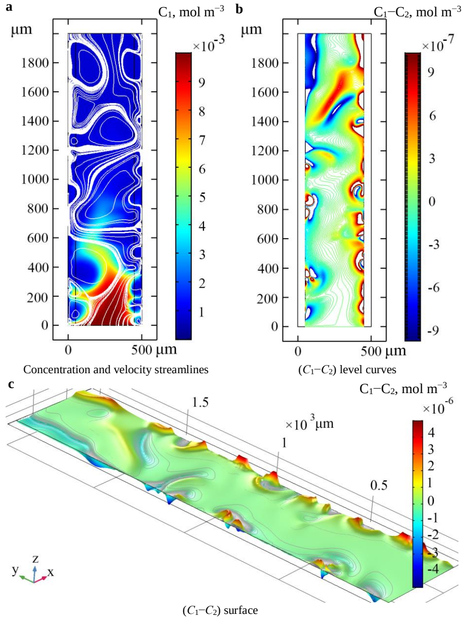
Fig. 11. The same as in Fig. 8; the results of simulation at |\Delta\phi|=2.973 V, t=594.5 s; space-charge breakdown: a positively charged SCR going from the CEM almost to the AEM (seen as a red band), section 6 in CVC (Fig. 7).
