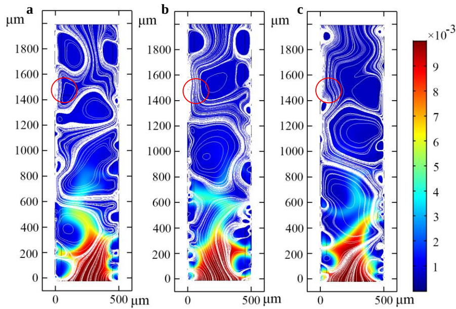
Fig. 13. Fluid streamlines at \Delta\phi=2.973 \text{ V} , t=594.5 \text{ s} (a); |\Delta\phi|=2.975 \text{ V} , t=595.0 \text{ s} (b) and |\Delta\phi|=2.978 \text{ V} , t=595.5 \text{ s} (c).
