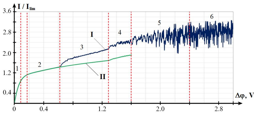
Fig. 7. Current-voltage characteristic of a membrane channel formed by an anion-exchange and cation-exchange membranes computed using the 2D model (curve I). A 0.01 \text{ mol m}^{-3} NaCl solution (viscosity 8.94 \times 10^{-4} \text{ Pa s} ) with an average velocity of 0.1 \text{ mm s}^{-1} flows; potential difference is swept with a rate of 5 \text{ mV s}^{-1} . Different regions of the CVC are shown: 1 – initial linear region; 2 – plateau of limiting current; 3 – unstable EC vortices occur only at the CEM; 4 – unstable EC vortices occur both at the CEM and AEM without overlapping these two vortex zones; 5 – collisions of the EC vortices and overlapping of vortex zones at the CEM and AEM, isolated cases of “global” space-charge breakdown; 6 – chaotic interaction of EC vortices, regularly repeated cases of “global” space-charge breakdown. Curve II is calculated for the solution viscosity 8.94 \times 10^{-3} \text{ Pa s} , which makes it possible to be almost totally suppress electroconvection.
