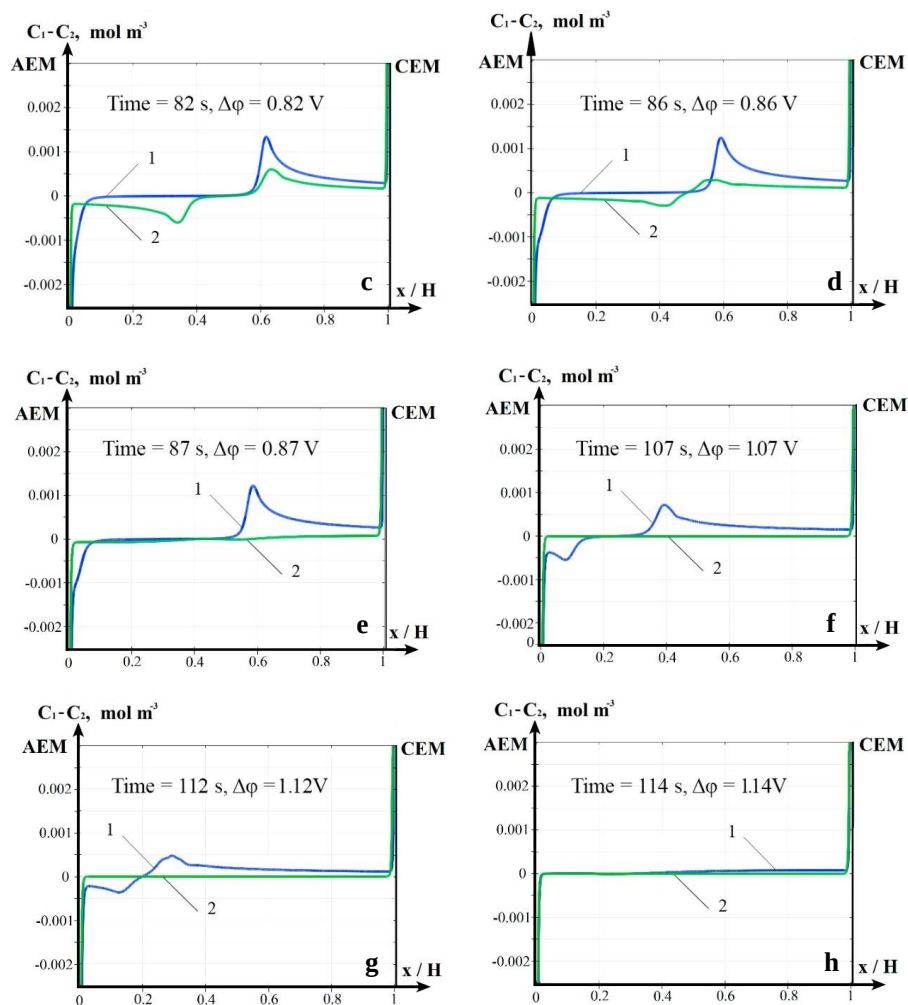
Fig. 4. Distribution of the space charge density in the solution between an AEM and a CEM; d=10 \text{ mV s}^{-1} ; C_0=0.1 \text{ mol m}^{-3} . The blue curve (1) corresponds to the NaCl solution, and the green curve (2), to KCl.
