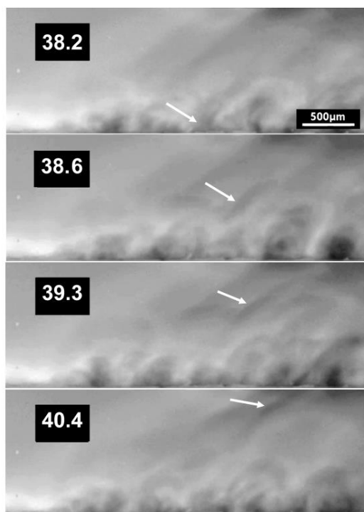
Fig. 14. Distribution of rhodamine concentration near an AMX-Sb anion-exchange membrane in electrodialysis of a 0.02 M NaCl + 10 \mu M rhodamine solution. Dark areas correspond to a low rhodamine concentration; light ones, to a high concentration.
