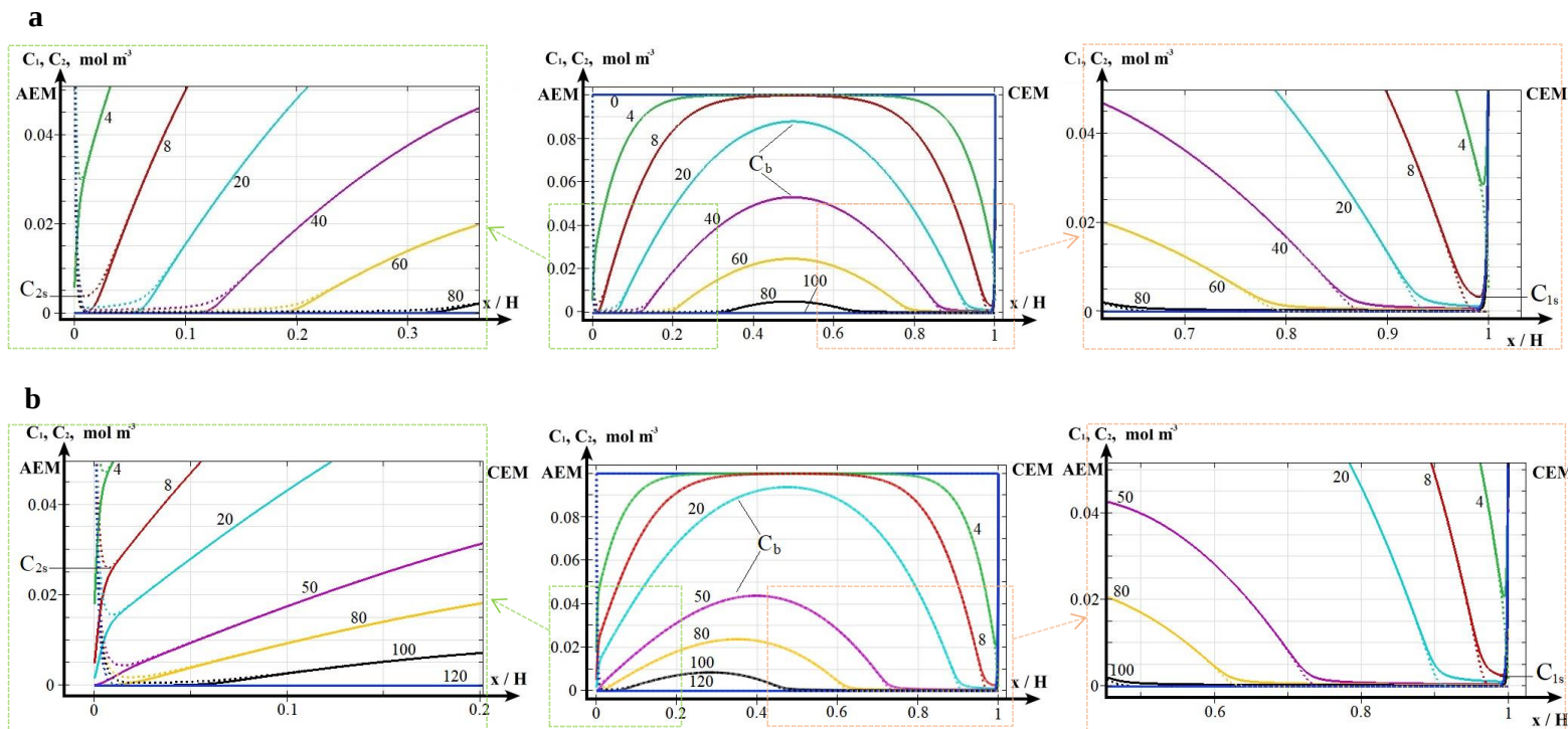
Fig. 3. Concentration profiles of cations (solid lines) and anions (dashed lines) in the cases when initially 0.1 \text{ mol m}^{-3} solution of KCl (a) or NaCl (b) are placed between an anion-exchange membrane (AEM) and a cation-exchange membrane (CEM) forming a dilute compartment of a non-flowing cell. Full-scale profiles are shown in the middle of the figure; on the left, there is the magnification of the area near the AEM; on the right, the magnification near the CEM. The results of calculations using Eqs. (1)-(7) (1D model), when a linear sweep of potential difference with a rate d=10 \text{ mV s}^{-1} is applied. The numbers at the curves show the time elapsed after the current is switched on; at the indicated times, the absolute value of the potential difference |\Delta\phi| is 0, 0.04, 0.08, 0.2, 0.4, 0.6, 0.8 and 1 (V), respectively. H=1000 \text{ }\mu\text{m} , C_{1m}=C_{2m}=0.1 \text{ mol m}^{-3} . The counterion transport number in both membranes is set equal to 1, since the solution is very dilute.
