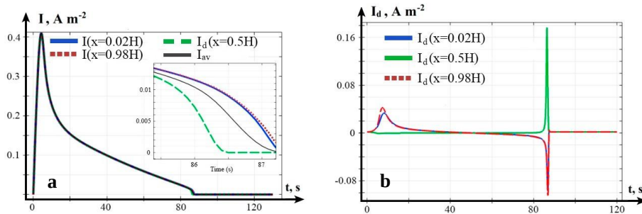
Fig. 5. Ionic conductance, I (a), and charging, I_d (b), current densities computed in the case of KCl at x=0.02H , 0.5H and 0.98H ; d=10 \text{ mVs}^{-1} , C_0=0.1 \text{ mol m}^{-3} .
