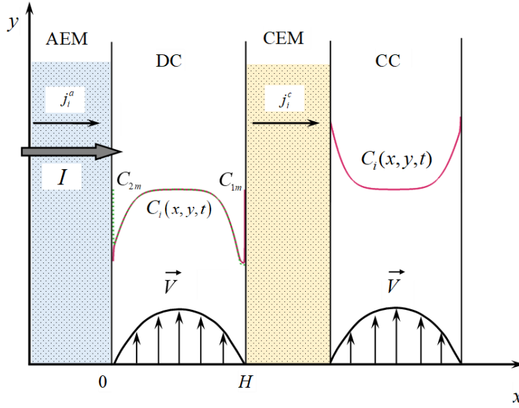
Fig. 6. 2D membrane system under study. Only the diluate compartment (DC) (the region between x=0 and x=H ) is considered; concentration profiles here are calculated, the solid line corresponds to the cation, the dashed line, to the anion. The concentration profile in the concentrate compartment (CC) is shown schematically. The parabolic distribution of velocities, \vec{V} , is assumed at the DC entrance. The counterion concentration is set at the membrane surfaces.
