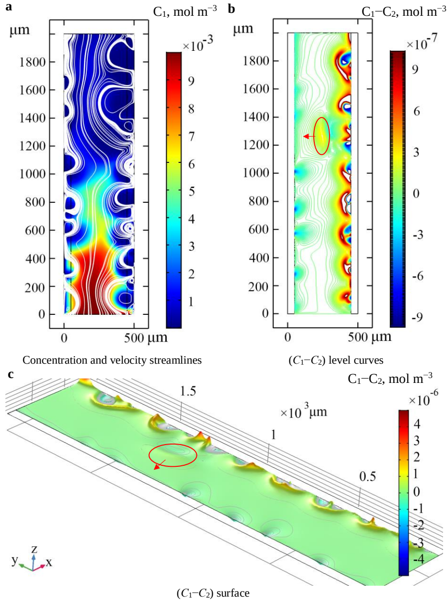
Fig. 10. The same as in Fig. 8; the results of simulation at |\Delta\phi| = 2.08 \text{ V} , t = 416 \text{ s} ; a local maximum of the space charge density (circled with a red line) in movement from the CEM to the AEM, section 5 in CVC (Fig. 7).
