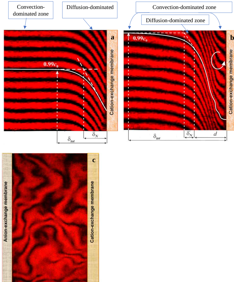
Fig. 2. Laser interferometric bands visualizing instantaneous concentration profiles (white lines) in flowing solution between a CEM and an AEM at underlimiting, i=0.5 i_{lim} (a), and overlimiting, i=2 i_{lim} (b), i=10 i_{lim} (c) current densities. The concentration profile in (a) agrees with the classical theory of ED [38]. The EC vortices at overlimiting currents disturb the concentration profiles (b, c). Redrawn from [16].
