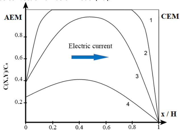
Fig. 1. Concentration profiles in the desalination compartment of an ED cell calculated (at a voltage 0.2 V, a NaCl solution) using the convection-diffusion model [38] at different dimensionless distances from the channel entrance Y = LD / (\bar{V}H^2) : 1 – 0, 2 – 0.001, 3 – 0.02, 4
