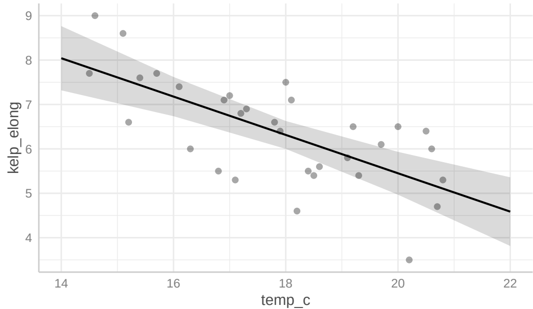
Predicted values of kelp_elong
