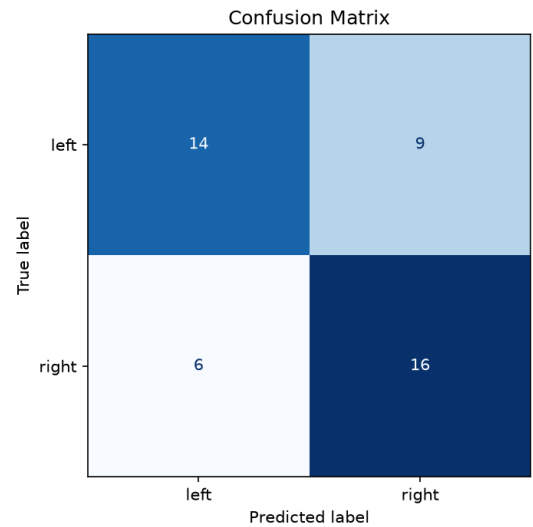
Fig. 5. Aggregated confusion matrix (5-fold stratified cross-validation).
