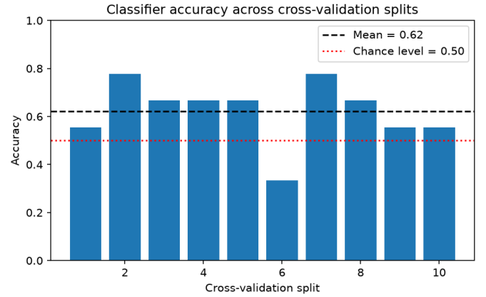
Fig. 4. Classification accuracy for each of the 10 cross-validation splits, relative to the mean (dashed) and chance level (dotted).
