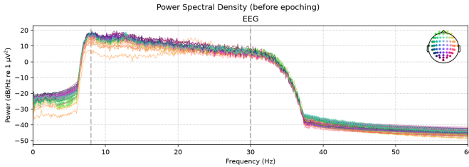
Fig. 2. Power spectral density (PSD) across all 64 EEG channels, prior to epoching.
