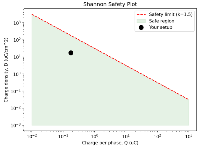
Fig. 2. Shannon safety plot: charge density vs. charge per phase (log-log axes), with the k = 1.5 safety boundary and the evaluated configuration marked.
