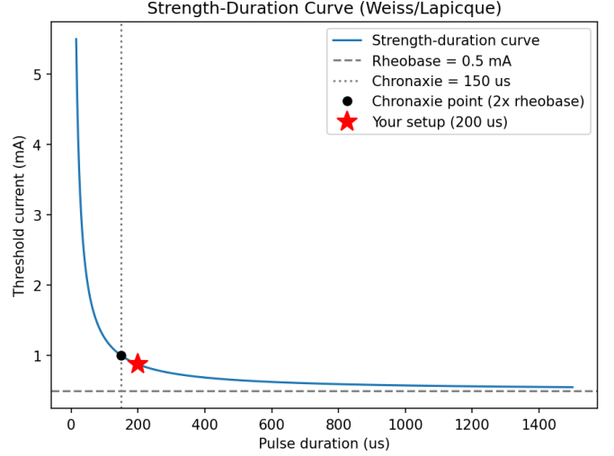
Fig. 1. Strength-duration curve for the example configuration (rheobase = 0.5 \text{ mA} , chronaxie = 150 \mu\text{s} ), with the chronaxie point and the evaluated 200 \mu\text{s} pulse duration marked.
