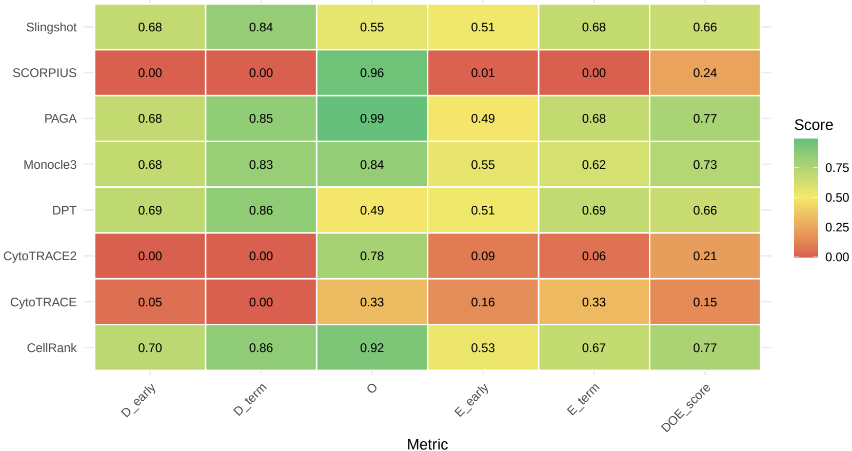
DOE Metrics Heatmap
