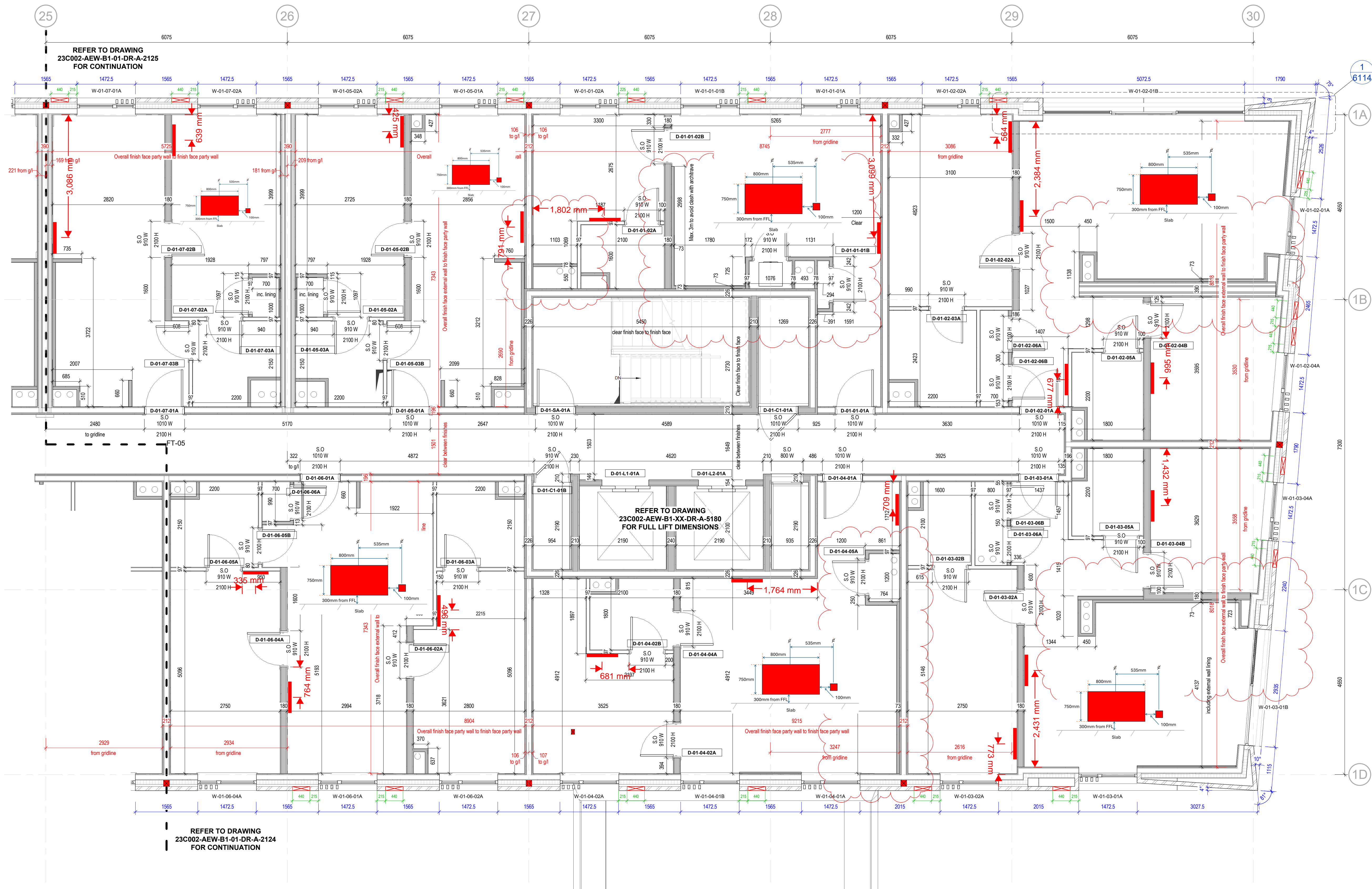
First Floor Plan Scale @ 1 : 50
