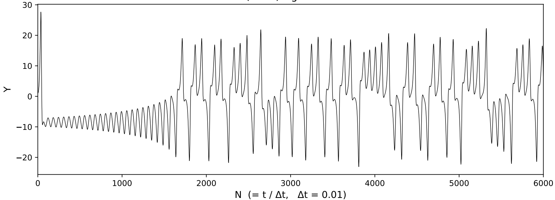
Lorenz (1963) Figure 1 — Y vs N
