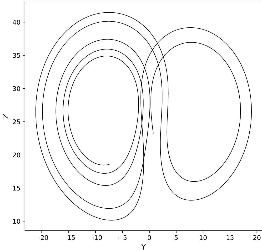
Lorenz (1963) Figure 2 — Z vs Y ( t \in [14, 19] )
