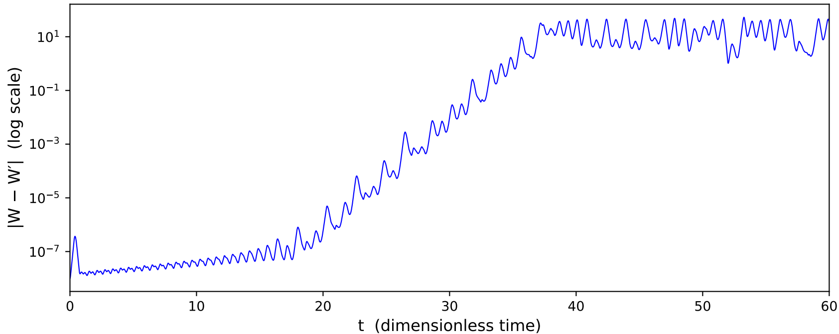
Sensitivity to initial conditions: distance between trajectories
