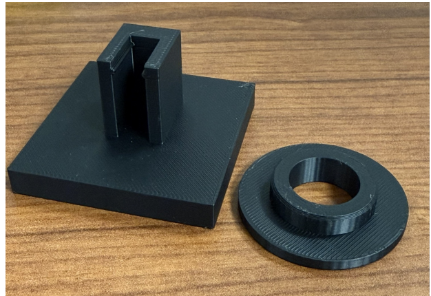
Nest and locating ring, as printed. The slotted nest sits on a wide base that registers flat to the platen. The ring is a separate locating feature printed alongside it.
