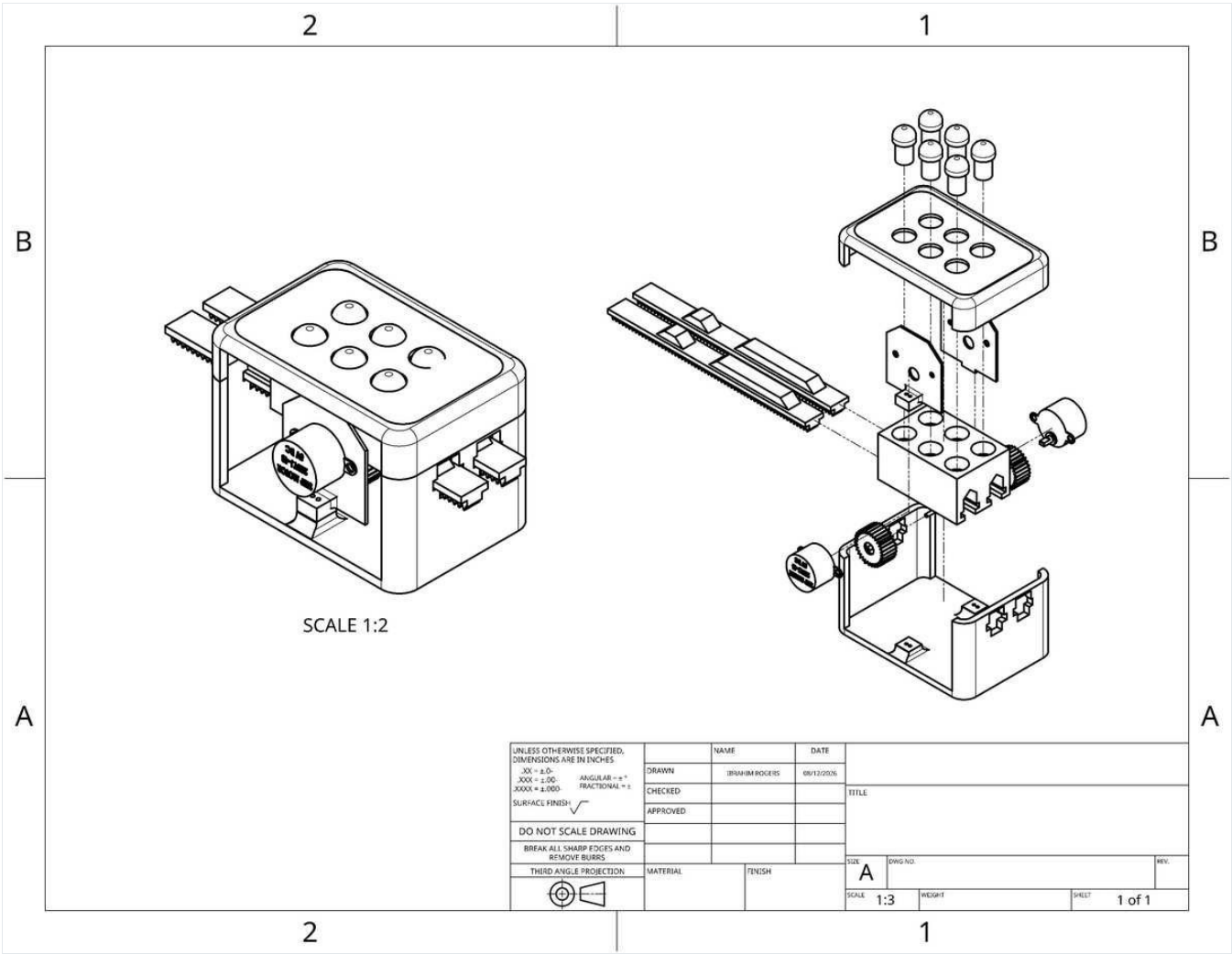
Top-level assembly drawing. Left: assembled enclosure (Scale 1:2). Right: exploded view (Scale 1:3) showing the six dome pins, letter-housing insert, guide bracket, pin-guide block, drive motor and pinion, rack, and enclosure top/bottom. Self-authored release drawing, dimensioned in inches per standard third-angle projection.
