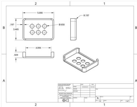
Enclosure top cover. 5.000 × 3.465 in with six Ø.650 in access holes for the dome pins and R.197 in corner fillets. Mounting flange at .929/4.094 in locates the cover to the bottom chassis.
