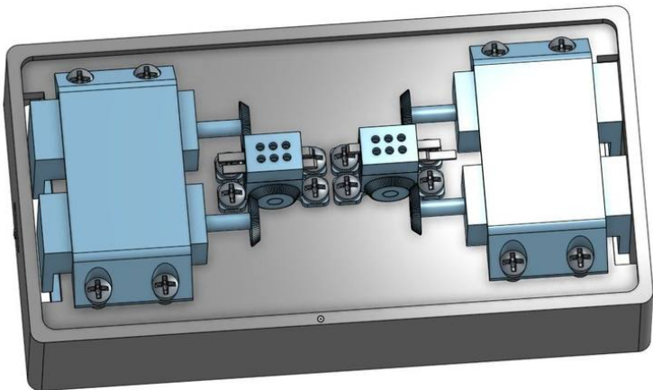
Two-cell assembly. Cells sit adjacent at reading pitch with motors outboard and racks driving inward. Each cell is independently addressed, so a character can be rewritten without disturbing its neighbor.
