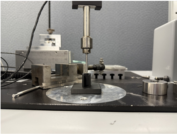
Nest in the load frame. Printed nest locating a molded component under the probe during sealing-force characterization. The slot constrains the part laterally while leaving the sealing face open.
