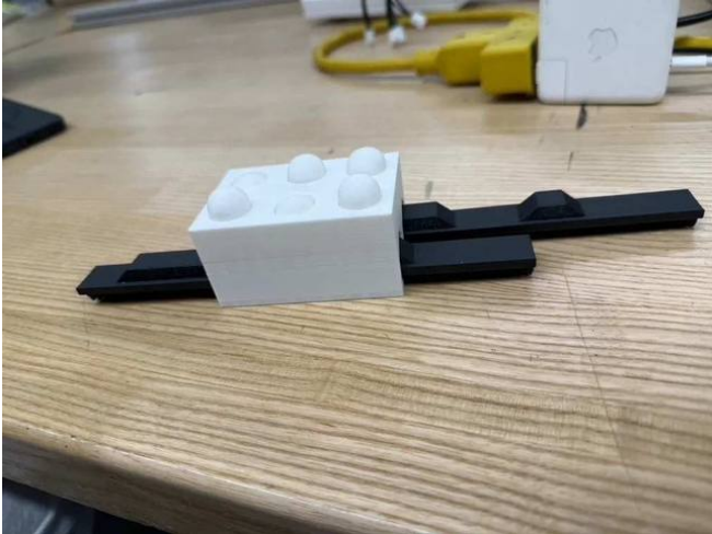
Assembled prototype — side view. White housing carries the pin actuation mechanism and rides on the black guide rails, which provide lateral constraint. Shows rail engagement and the travel available to the rack.
