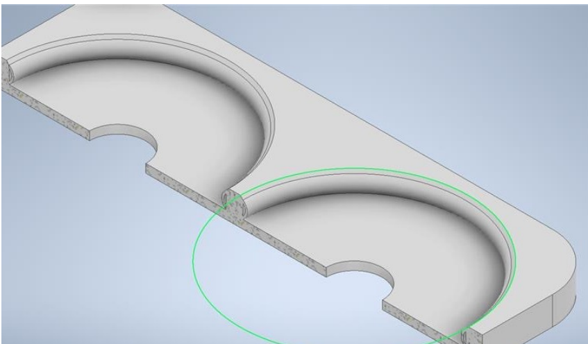
Two-pocket module. Each pocket carries a compliant retention wall around the recess. Modules butt together so a tray is built from repeated units rather than drawn at a fixed length.
