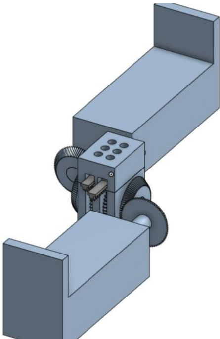
Single cell. The two racks enter from opposite faces, each driven by its own bevel gear. Rack channels extend away from the cell in opposite directions, which keeps the gearing and motors clear of the six-dot footprint.
