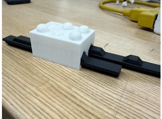
Front three-quarter view. Shows the six-dot face and the housing-to-rail interface where side-load binding originated. Lead-in chamfers on the rails were added at this interface to ease pin entry.
