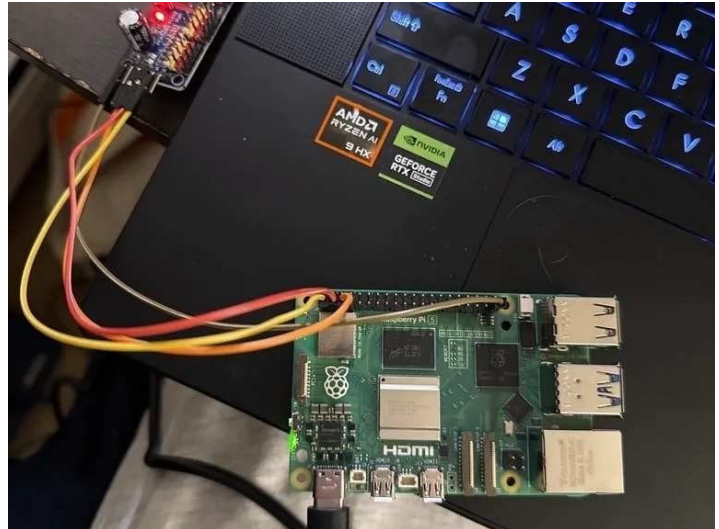
Electronics integration. Raspberry Pi 5 driving the PCA9685 servo controller over I 2 C, with servo power on a separate rail from compute power to keep actuation transients off the Pi.
