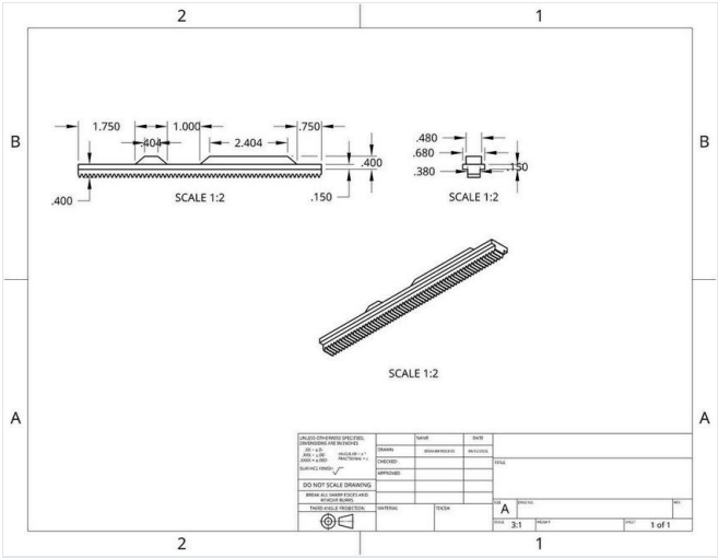
Stepped rack. Linear rack with two lead-in cam profiles at 1.000 in pitch (Scale 1:2), plus a keyed drive tab (.480/.680/.380 in, Scale 1:2) that engages the pin it lifts. This is the tolerated release version of the stepped-rack concept modeled earlier in Onshape.
