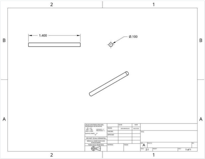
Guide dowel. Ø.100 in × 1.400 in ground pin. Locates the pin-guide block against the enclosure and keeps rack travel aligned under side load.
