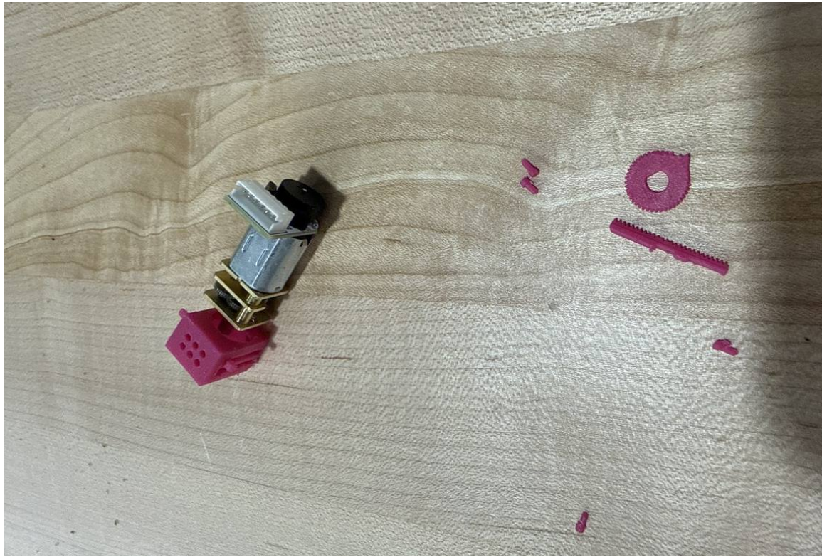
Production-scale cell, printed parts, and drive motor. The cell body sits on the output shaft of the gearmotor that drives it, with a rack, bevel gear, and dome pins alongside. Everything is shown at true relative scale, which is the point of the photograph: the drive hardware is larger than the cell it actuates.
