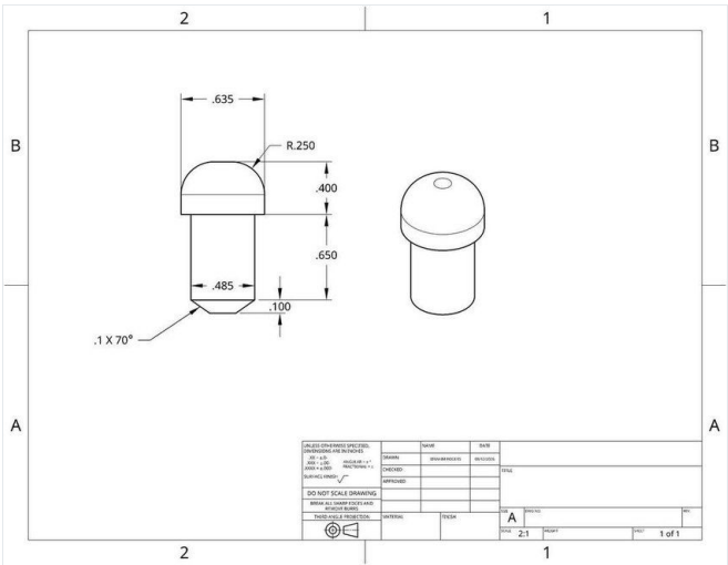
Dome pin. Ø.485 in shaft with a Ø.635 in domed head (R.250 radius) and a .1 × 70° lead-in chamfer at the tip. The shaft rides in the Ø.500 in bore of the pin-guide block, giving .015 in diametral clearance across the actuation stroke.
